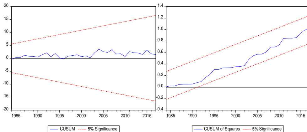
Figure 1. CUSUM Test Figure 2. CUSUMQ Test
