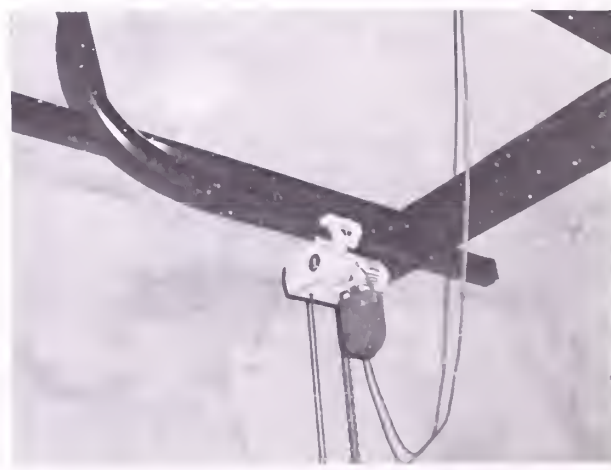
FIGURE 15.—Traveling electric chain hoist for handling a carcass during slaughter operations.
