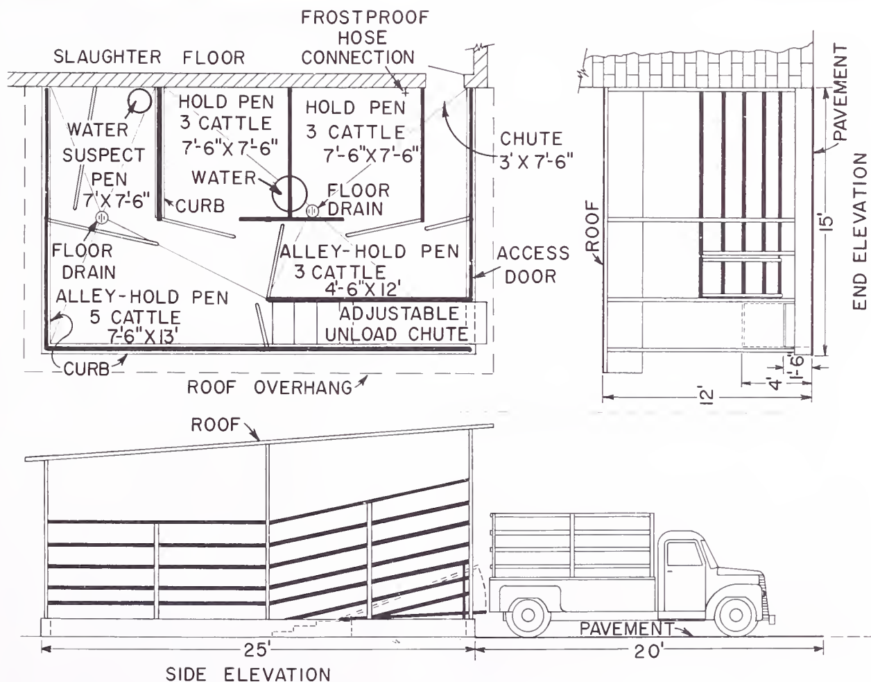
FIGURE 9.—Adjustable-height unload-chute and hold-pen layout.
