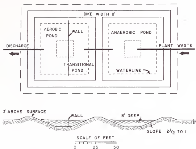
FIGURE 30.—Layout of a lagoon system.
