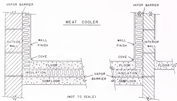
FIGURE 22.—Suggested method for constructing refrigerated room walls and floor.
