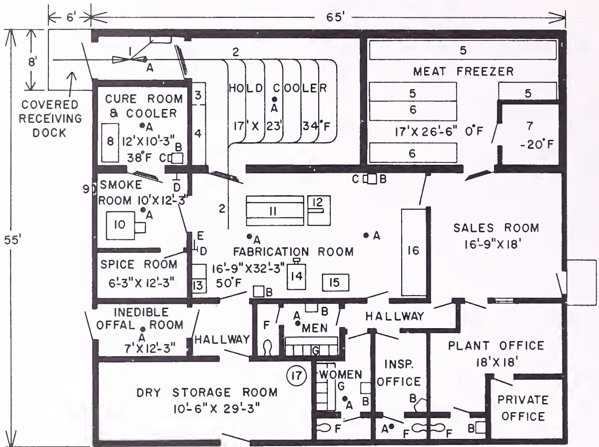
FIGURE 6.—Layout for a nonslaughter plant. (1) Track scale, (2) 7'6" high rail, (3) return product, (4) meat shelves, (5) meat baskets, (6) meat lockers, (7) quick freezer 8' x 8', (8) ham-pump table, (9) exhaust fan, (10) smokehouse, (11) boning table, (12) bandsaw, (13) sink, (14) meat grinder, (15) patty machine, (16) packing table, (17) water heater 140° F, (A) floor drain, (B) lavatory, (C) sterilizer, (D) hot and cold water, (E) thermometer in waterline, (F) toilet, and (G) clothing locker.
