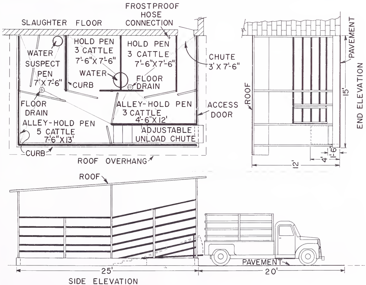
FIGURE 9.—Adjustable-height unloading chute and hold-pen layout.
