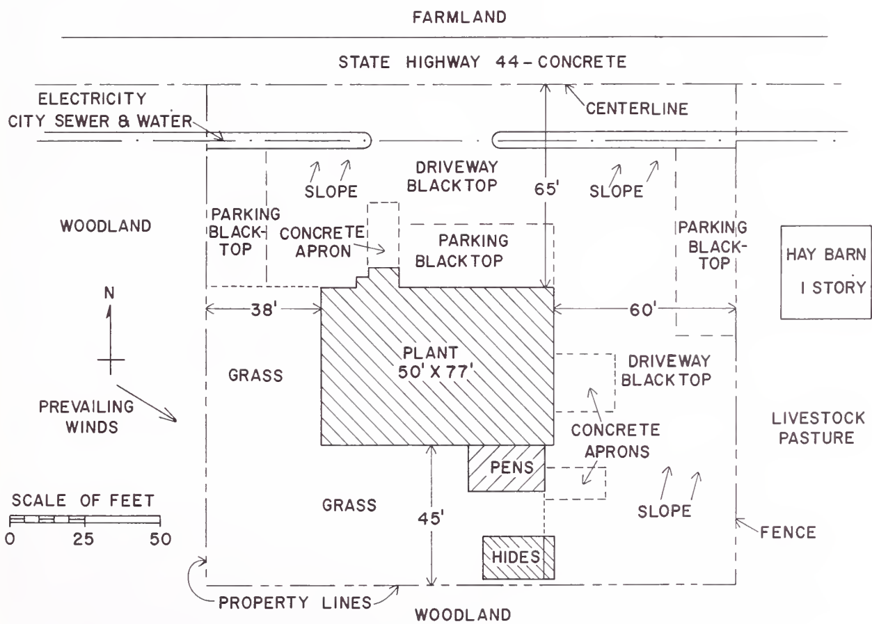
FIGURE 3.—Plot plan for a small slaughter plant.
