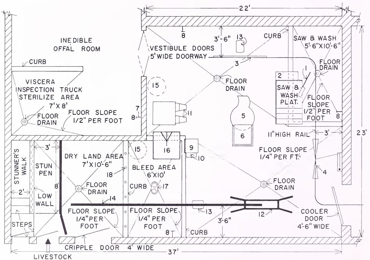
FIGURE 19.—Suggested layout for slaughter floor handling more than one head at a time, where all carcasses are skinned. (1) Carcass saw, (2) saw sterilizer, (3) carcass lander, (4) track scale, (5) viscera inspection truck, (6) inspection pan, (7) thermometer, (8) hot and cold water, (9) lavatory, (10) equipment sterilizer, (11) head inspection loops, (12) skinning cradle, (13) hoist, (14) I-beam 16' high, (15) inedible container, (16) head flush cabinet, (17) blood and water drain, and (18) safety fence.
