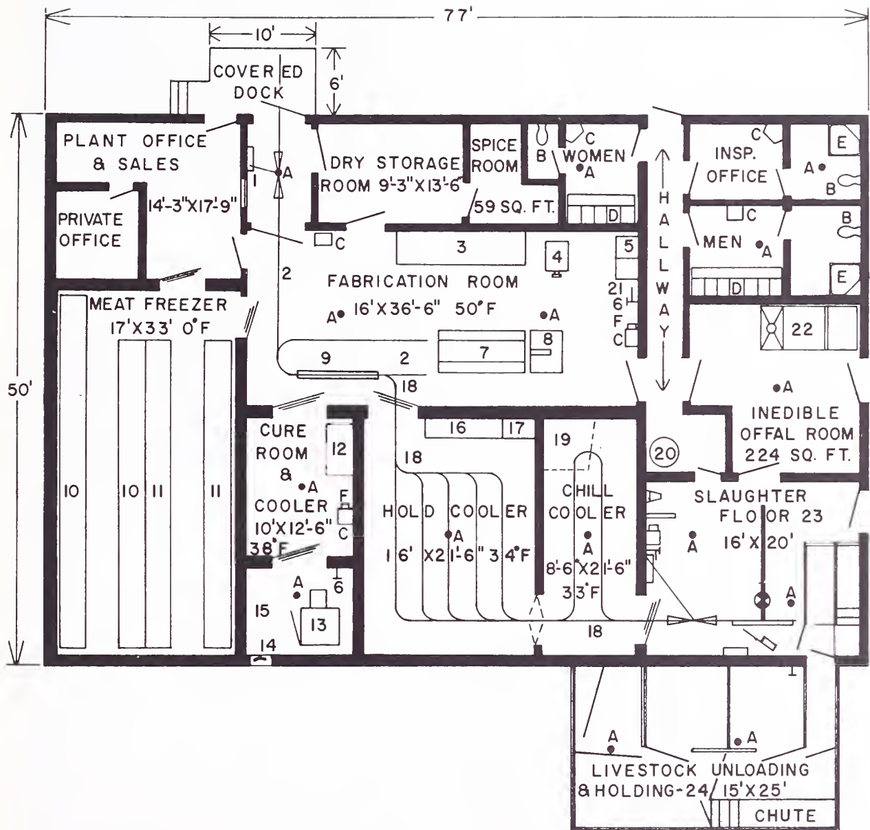
FIGURE 5.—Layout for a slaughter plant. (1) Track scale, (2) 7'6" high rail, (3) packing table, (4) meat grinder, (5) sink, (6) hot and cold water, (7) boning table, (8) bandsaw, (9) quarter dropper, (10) meat baskets, (11) meat lockers, (12) ham-pump table, (13) smokehouse, (14) exhaust fan, (15) smoke room 8' x 10', (16) meat shelves, (17) return products, (18) 11' high rail, (19) collapsible retaining cage, (20) water heater 180° F, (21) thermometer in waterline, (22) paunch work table, (23) details on figure 11, (24) details on figure 9, (A) floor drain, (B) toilet, (C) lavatory, (D) clothing locker, (E) shower, and (F) sterilizer.
