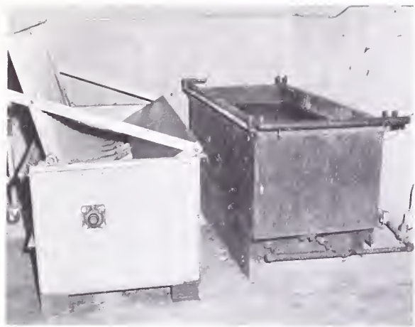
FIGURE 18.—Hog scald vat and dehairer in a small plant.
