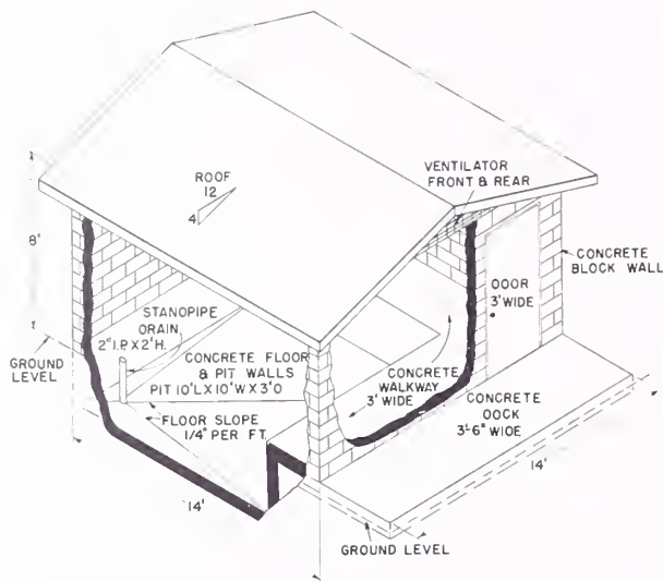
FIGURE 29.—Perspective drawing of a suggested hide house with a capacity of 300 hides.
