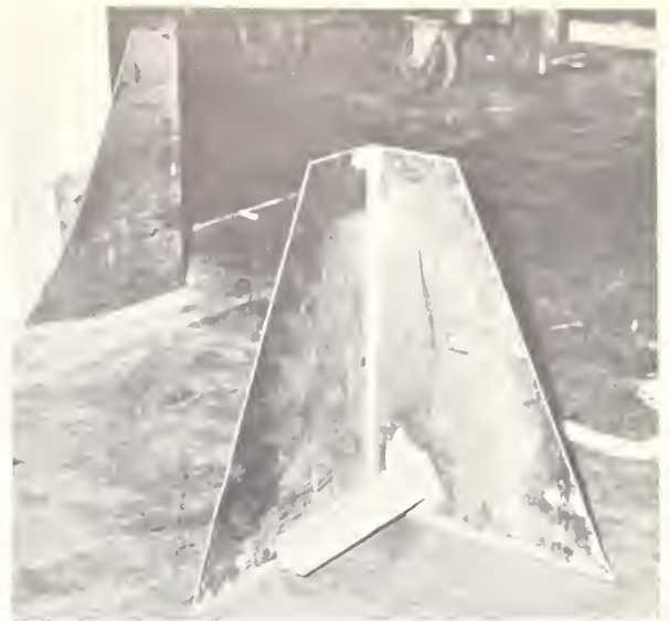
Figure 7.--(A) Metal guards used in one grocery warehouse for traffic corners; and (B) a closeup of the corner guards showing construction details.
