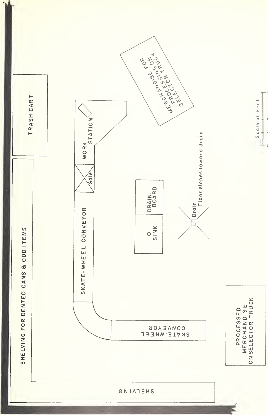
Figure 14.--A layout for a warehouse salvage operation.
