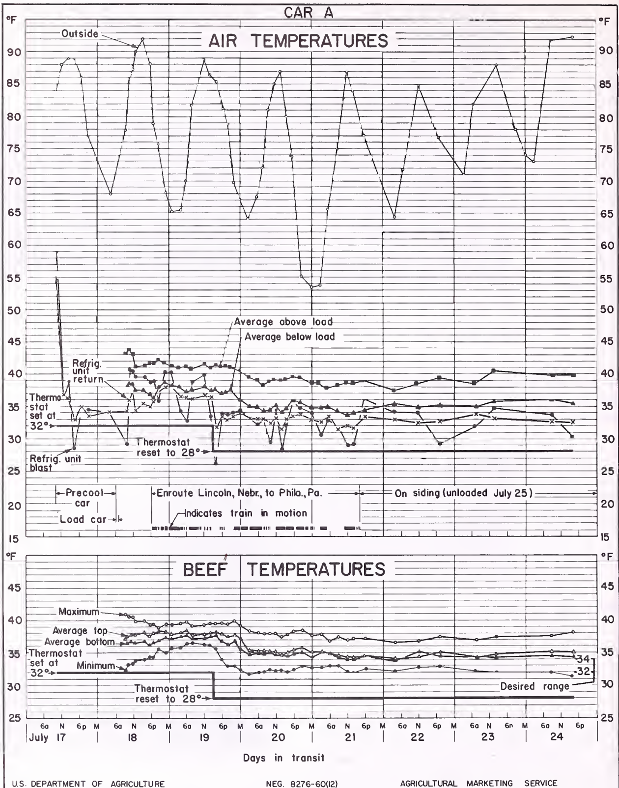
Figure 13.--Temperatures in car A which blasted air directly into load.
