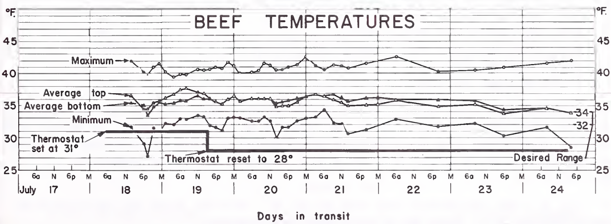
Figure 18.--Temperatures in trailer D which blasted air directly into load.
