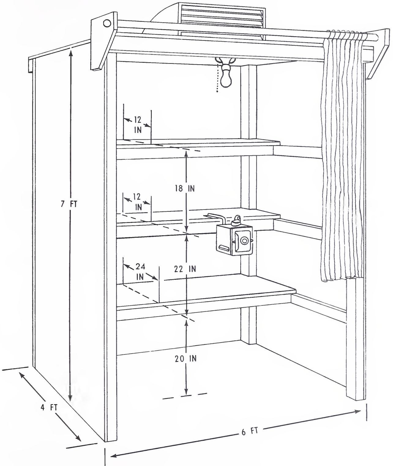
Figure 2.--Candling booth for periodically checking egg quality.
