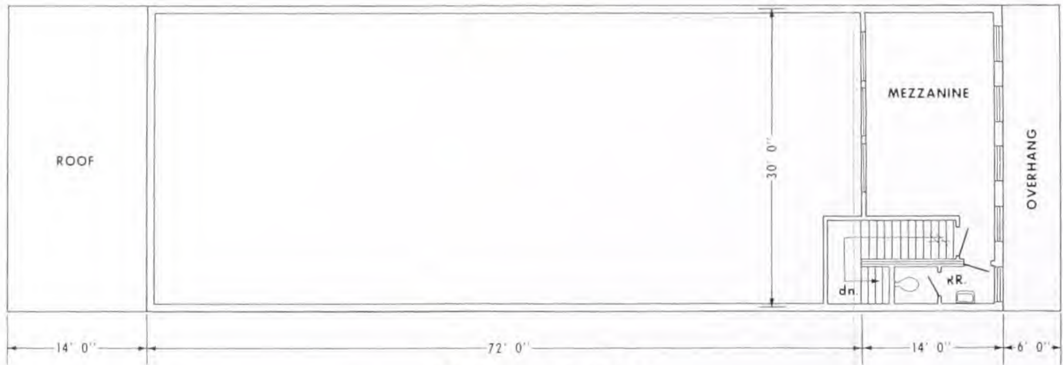
MEZZANINE PLAN
