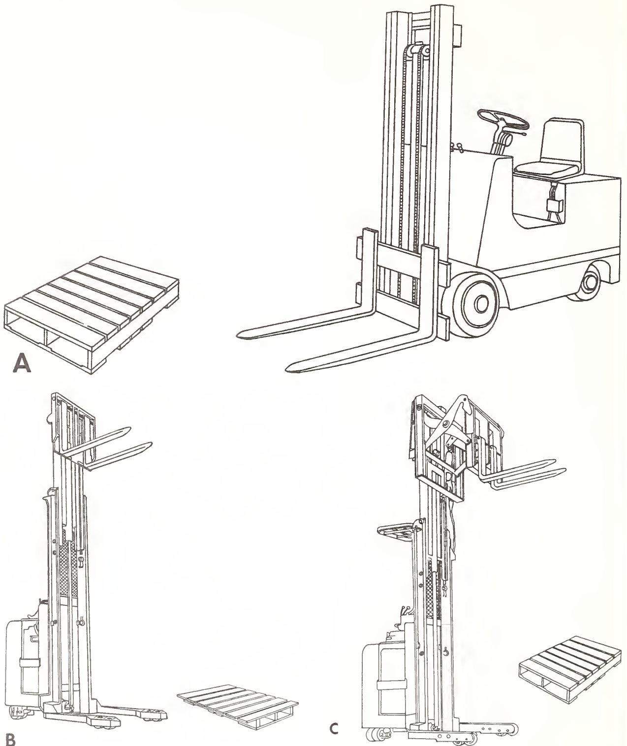
FIGURE 3.—Forklift trucks and pallets used in multiple-occupancy buildings: A, Counterbalanced forklift truck with conventional pallet; B, straddle forklift truck with single-wing pallet; C, extendable forklift truck with conventional pallet.
