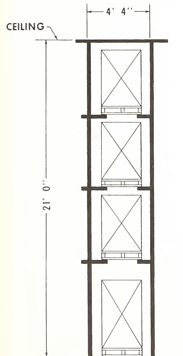
FIGURE 8.—Drive-through pallet rack.
