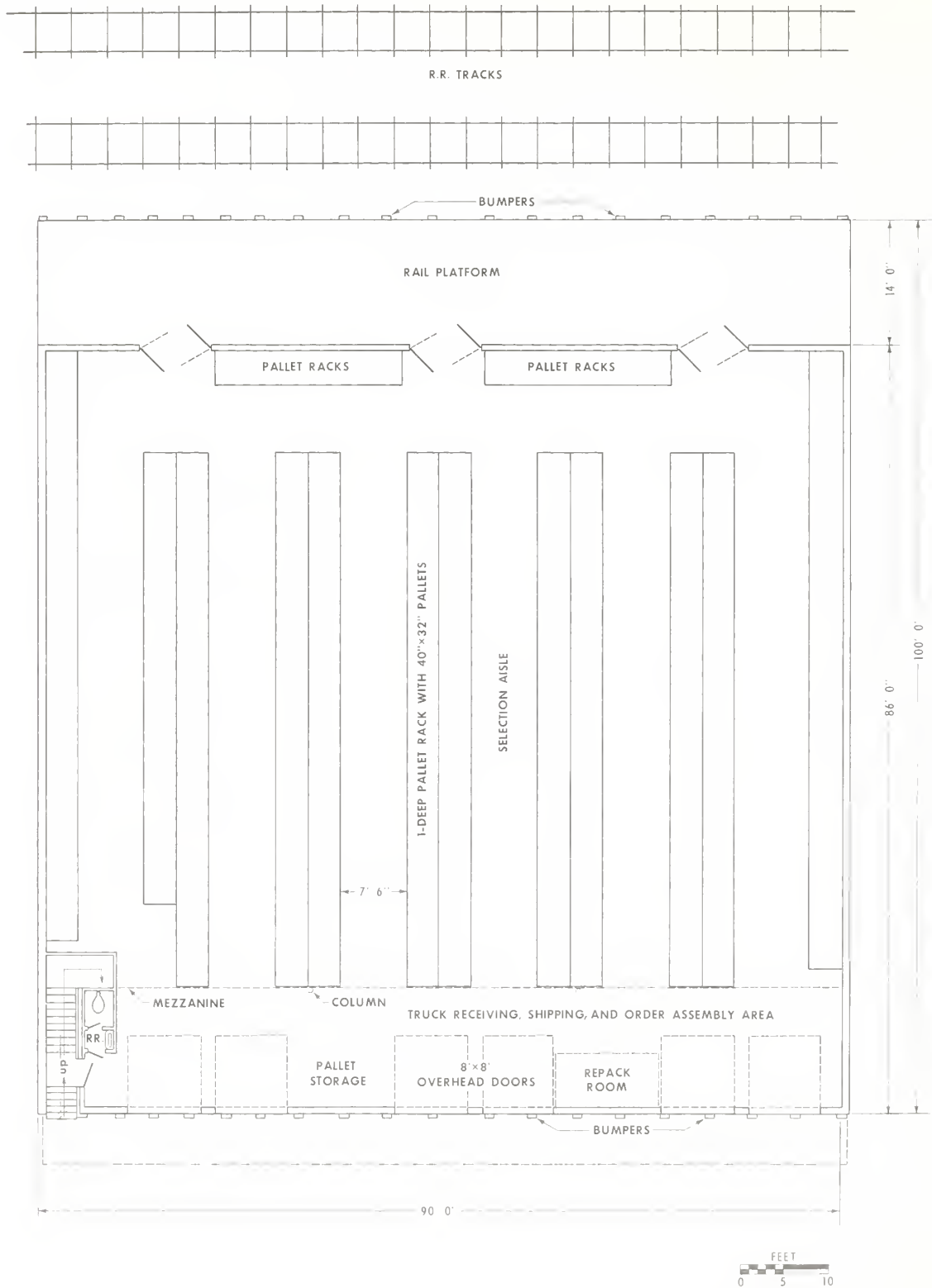
FIGURE 13.—Internal arrangement for an institutional wholesale grocery firm using three units of a multiple-occupancy building.
