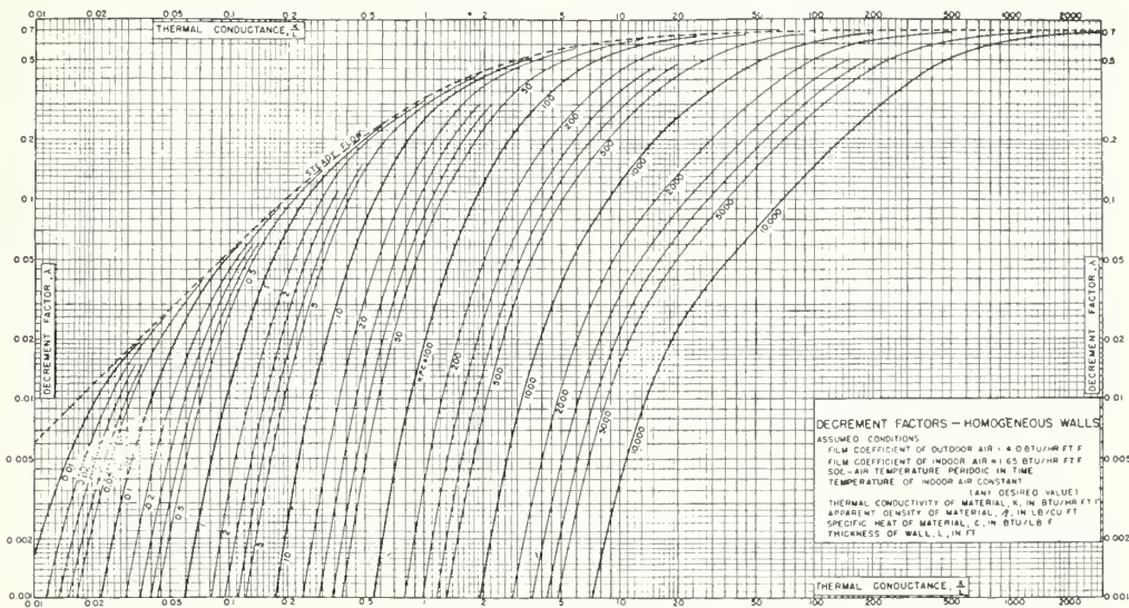
FIGURE 31.—Chart for determining decrement factors.
