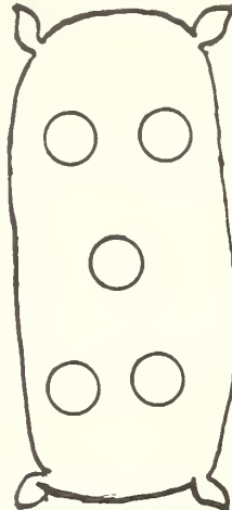
5-core side pattern for 3-inch tube
