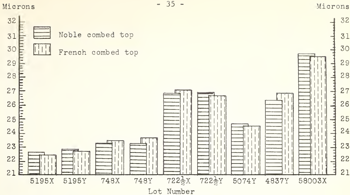
Figure 5.- The effect of Noble and French combing on the fineness of wool tops produced from the same original lot.
