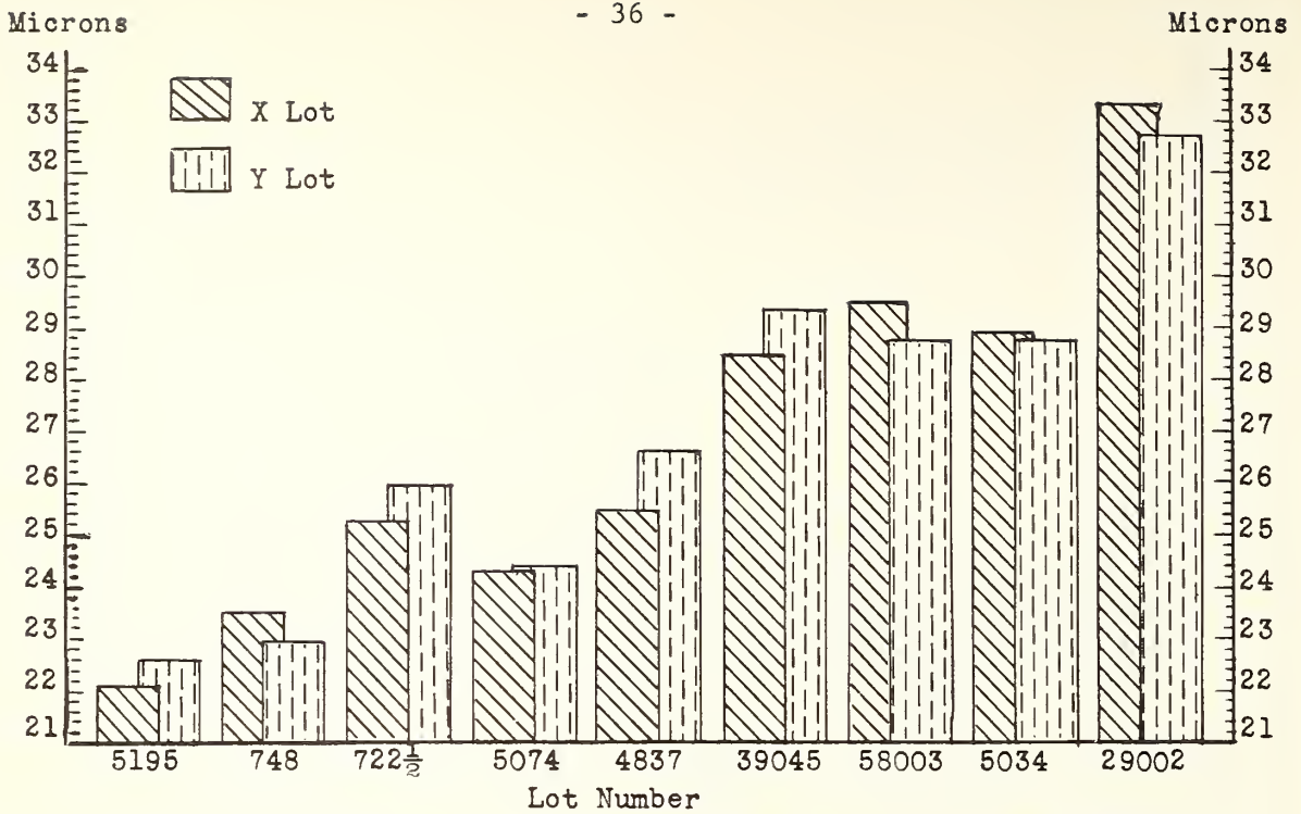
Figure 7.- The fineness of \frac{1}{4} -inch core samples drawn from the split (X and Y) lots.
