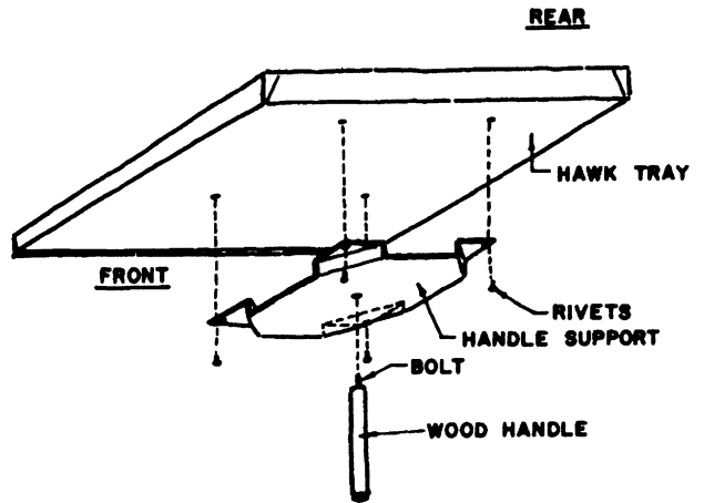
Figure 2.—Homemade hawk designed especially for surface-bonding work.
