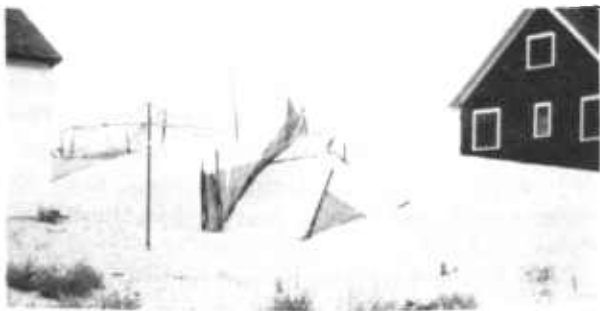
PN 1948 Sand dunes on coasts and lake beaches cause serious problems near summer cottages, and on highways and military installations. Control can be maintained in these locations through the planting of beach grass, the use of sand fences, and the application of hay mulches that contain an asphaltic adhesive.
