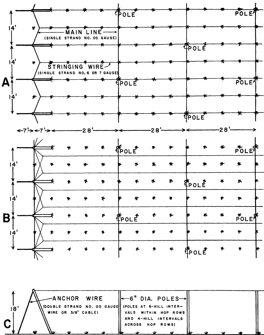
FIGURE 5.—Diagram showing common trellis designs on 7 foot by 7 foot spacing: (A), Stringing wires placed over rows; (B), stringing wires placed over centers; (C), side elevation showing system of anchoring used on edges of yard.
