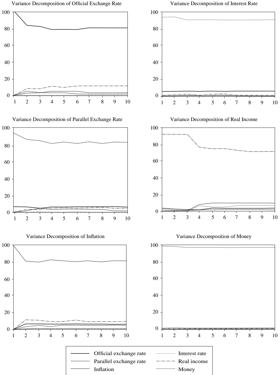
Fig. 2. Variance Decomposition from the Reduced-Form Model
