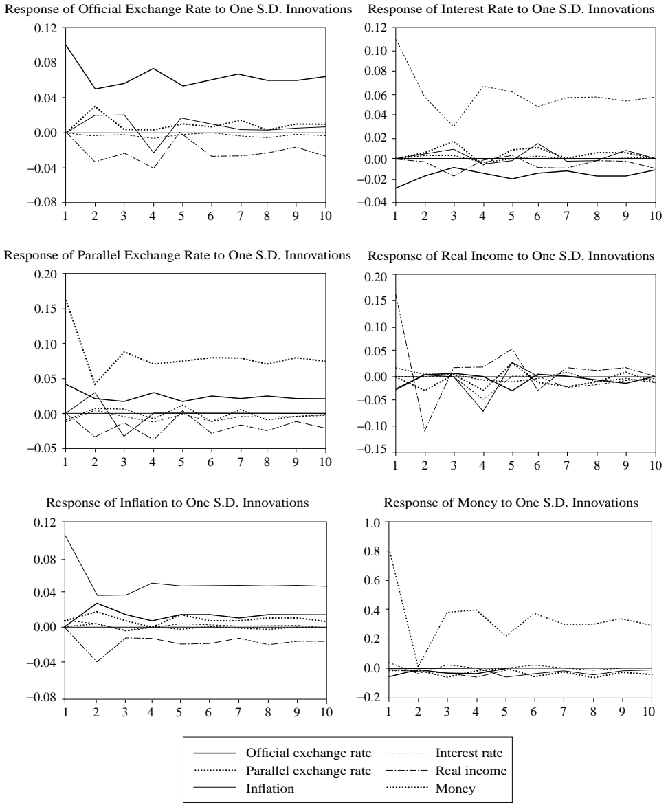
Fig. 1. Impulse Response Functions
