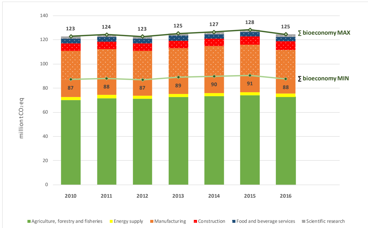
Figure 3.17. Structure of greenhouse gas emissions of German bioeconomy
