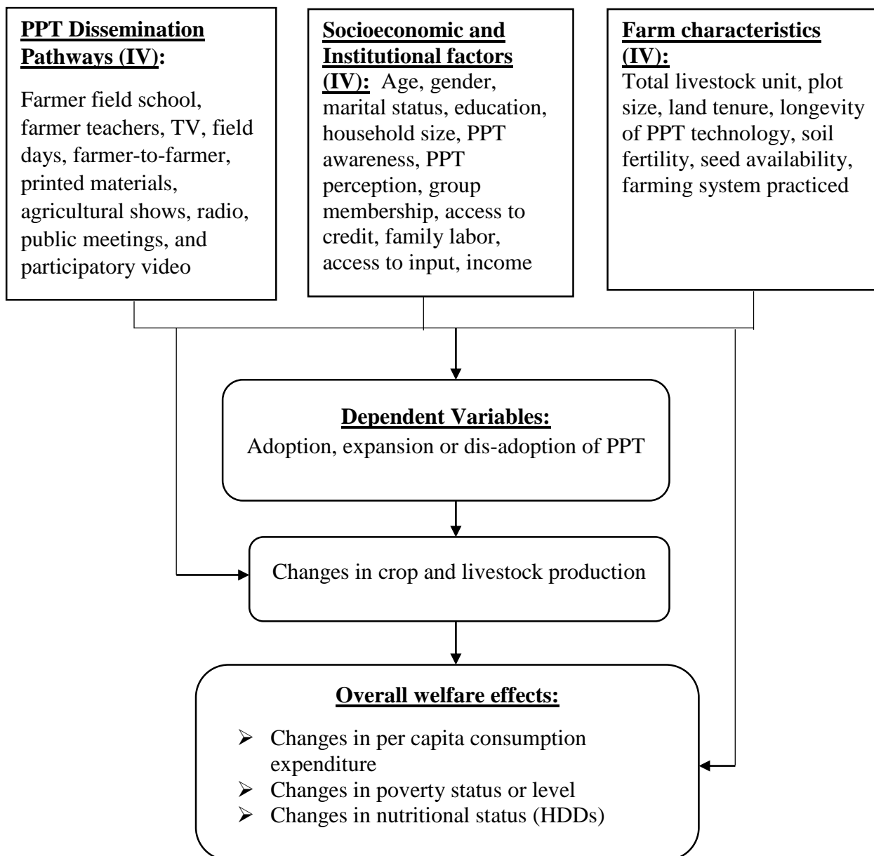
Figure 1: Conceptual Framework
