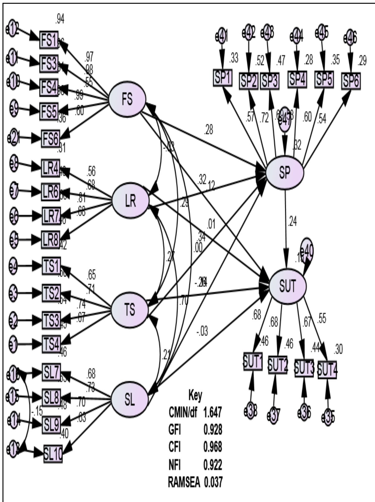
Figure: 2: The SEM Full Structural Model for the Overall Sample
