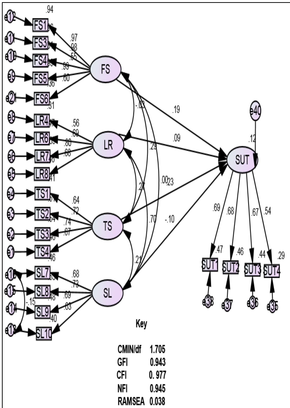
Figure 2. SEM Direct Effect Without mediator
