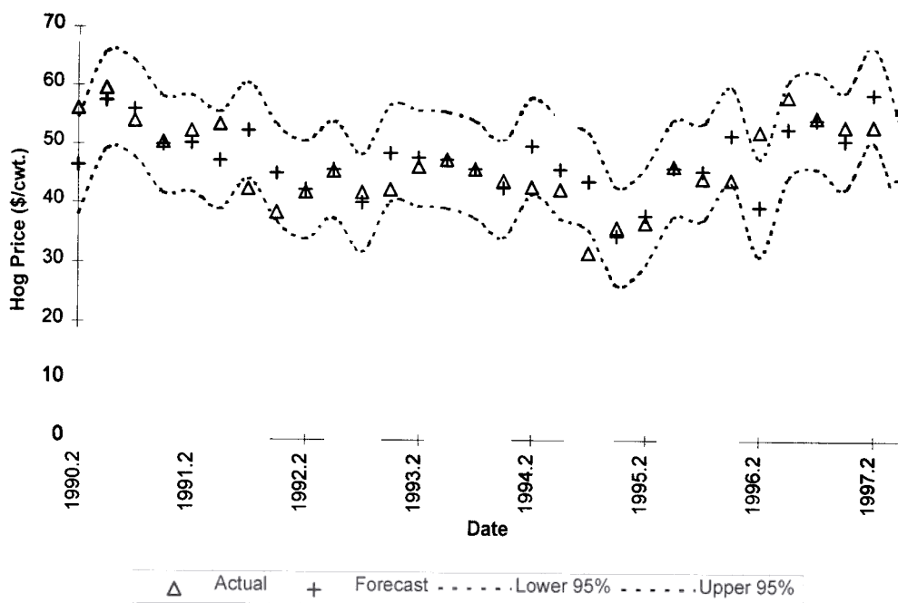
Figure 3. Forecasts from ARIMA model using fixed coefficients
