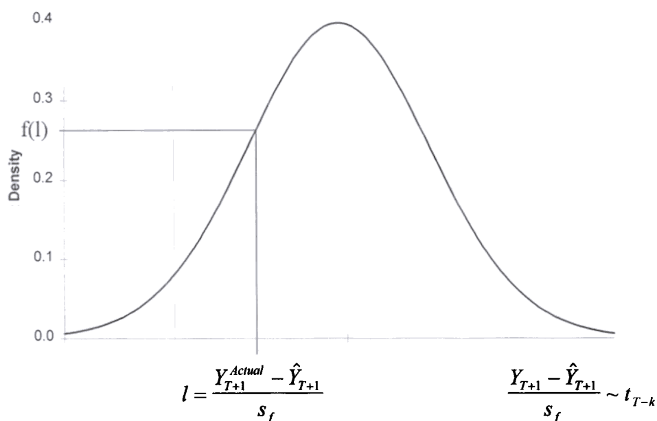
Figure 1. Illustration of likelihood score for a single forecasted point
