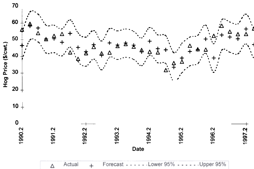
Figure 5. Forecasts from ARIMA model using quarterly updated coefficients
