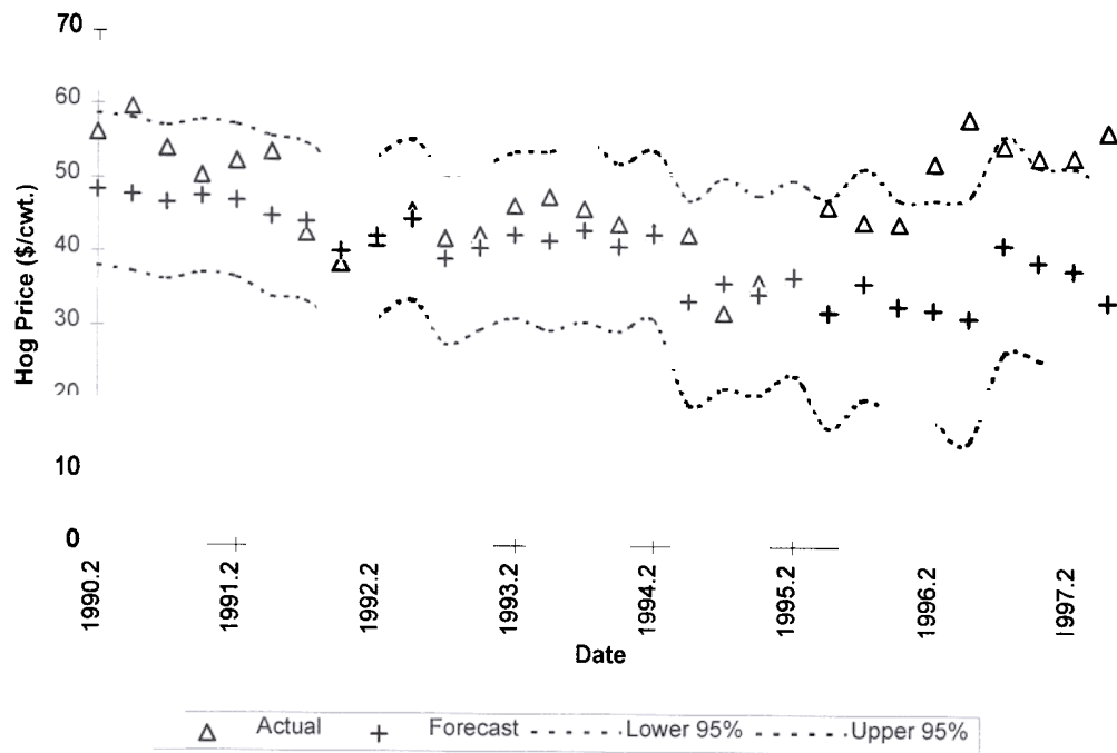
Figure 2. Forecasts from econometric model using fixed coefficients
