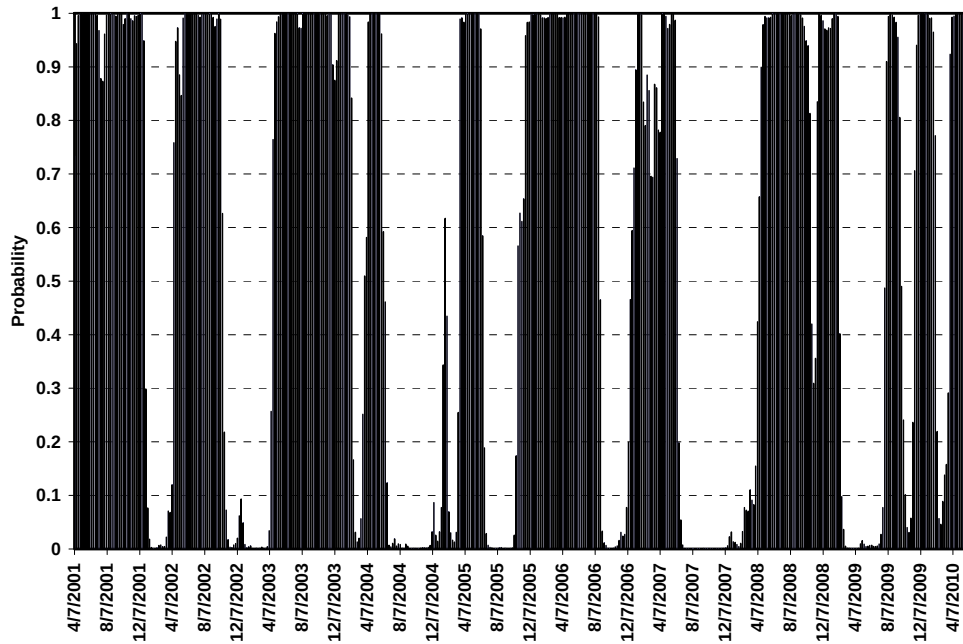
Figure 3: Probability of cooperative regime, April 2001 – May 2010. (Shaded regions identify periods of cooperative regime.)
