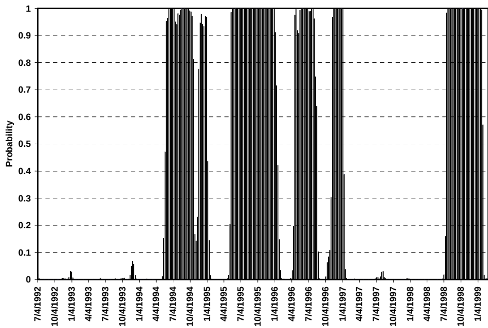
Figure 4: Probability of cooperative regime, July 1992 – February 1999. (Shaded regions identify periods of cooperative regime.)
