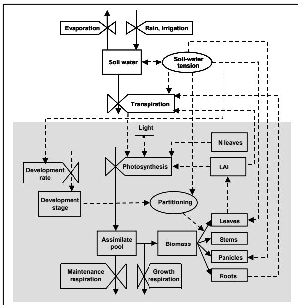
Fig. 3.1B. For the situation of water-limited production, ORYZA1 (gray area) and its links to the water balance sub-routines.
