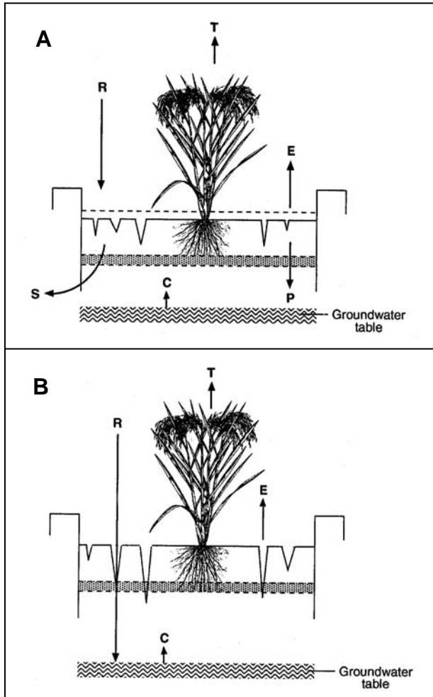
Fig. 6.2. Vertical profile and water balance of puddled soil with cracks. In (A), cracks have not yet extended through the plow sole; in (B), cracks have penetrated into the subsoil. E = evaporation, P = percolation, R = rainfall, S = seepage, C = capillary rise, and T = transpiration.
