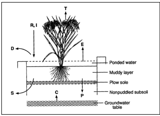
Fig. 6.1. Vertical profile and water balance of puddled soil. D = surface drainage, E = evaporation, I = irrigation, P = percolation, R = rainfall, S = seepage, T = transpiration, C = capillary rise from the groundwater table.
