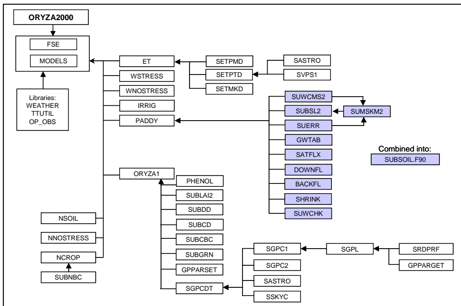
Fig. 2.1. Program and library structure of ORYZA2000 in the FSE system.
