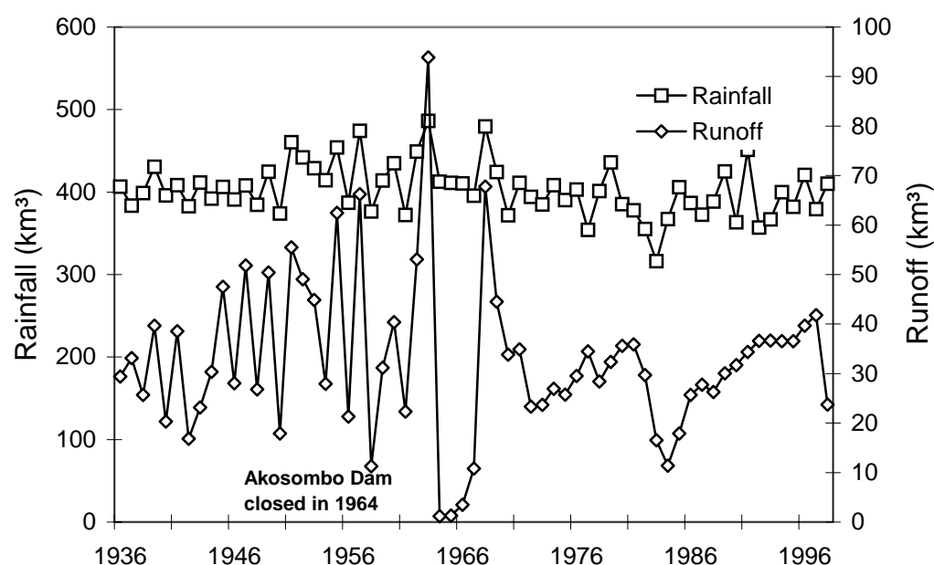
Figure 1: Water Balance
