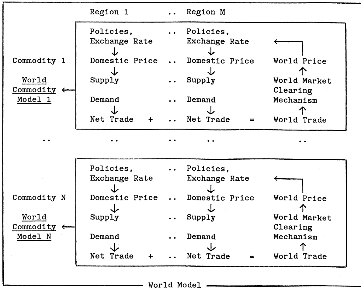
Figure 1--Structure of SWOPSIM Models
