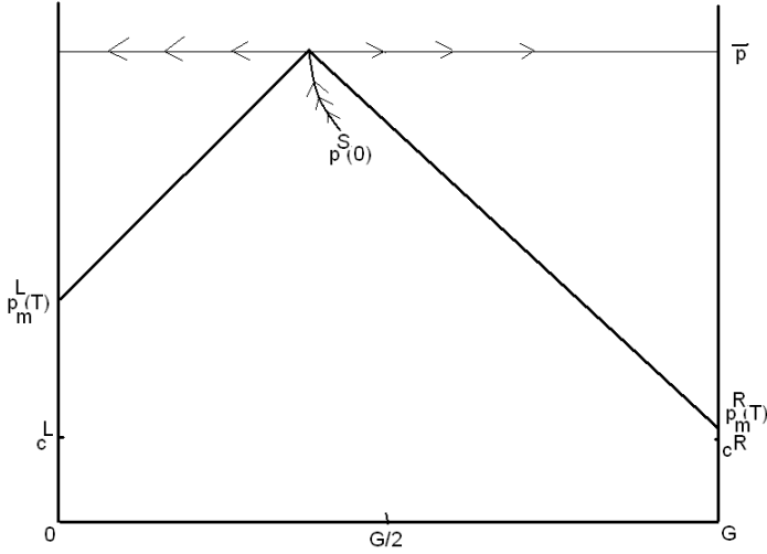
Figure 1: p^S(0) moves up to \bar{p} over Phase I. Each supplier extracts in isolation in Phase II.
