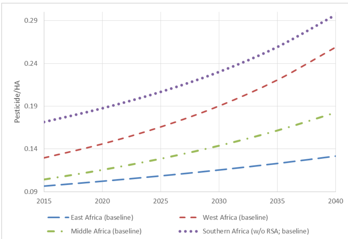
Figure 2. Projected average total pesticide use (Kgs a.i. /ha) for SSA and by region (baseline growth)
