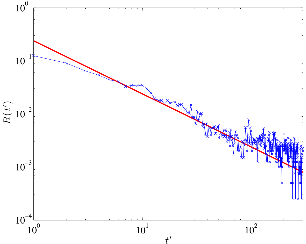
Figure 4: The autocorrelation function of the binary representation of default events S(t) (blue diagonal crosses). The analytical prediction given by Eq. (23) is also shown (red solid line).
