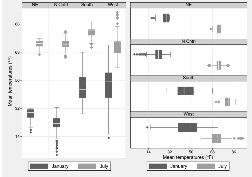
Figure 2. Box plots for January and July temperatures of various U.S. cities using the by() option to compare different regions
