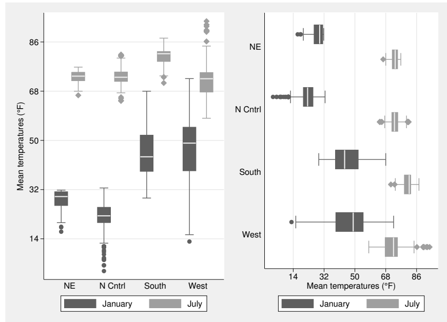
Figure 1. Box plots for January and July temperatures of various U.S. cities using the over() option to compare different regions
