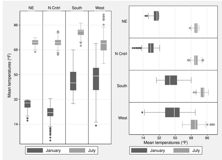
Figure 3. Box plots for January and July temperatures of various U.S. cities using the by() option to compare different regions, but with panel titles shown differently
