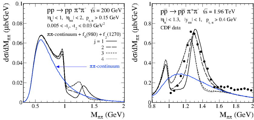
Figure 3: Two-pion invariant mass distribution for the STAR [5] (left) and CDF [6] (right) kinematics. The individual contributions of different IPf_2 couplings ( j = 1, \dots, 4 ) are compared with the CDF data [6]. The Born calculations for \sqrt{s} = 200 GeV and \sqrt{s} = 1.96 TeV were multiplied by the gap survival factors \langle S^2 \rangle = 0.2 and \langle S^2 \rangle = 0.1 , respectively. The blue solid lines represent the non-resonant continuum contribution only ( \Lambda_{off,M} = 0.7 GeV) while the black lines represent a coherent sum of non-resonant continuum, f_0(980) and f_2(1270) resonant terms.
