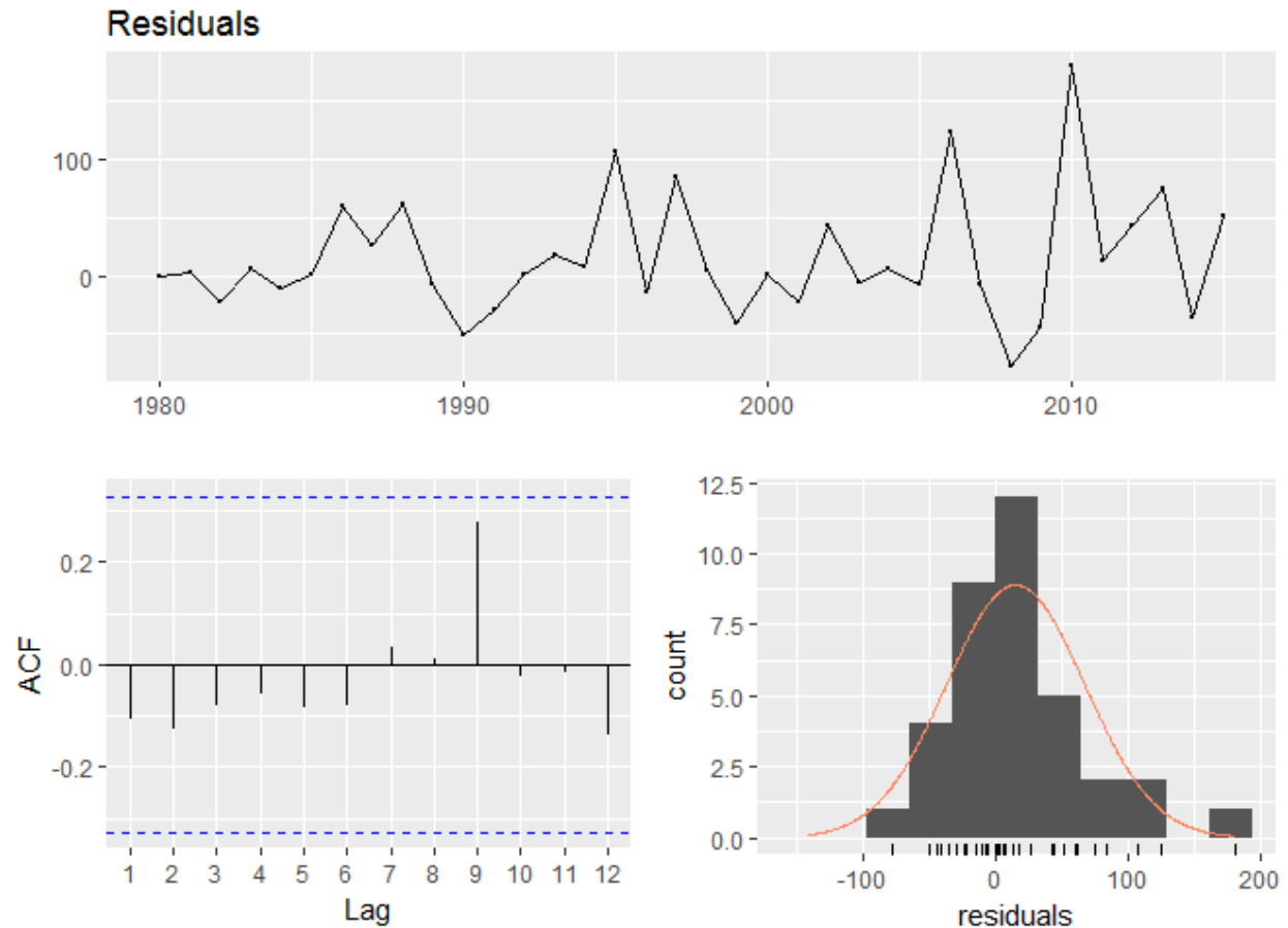
Figure 15. Residual analysis of domestic food utilization of dry peas and lentils' ARIMA (4,1,3) model.
