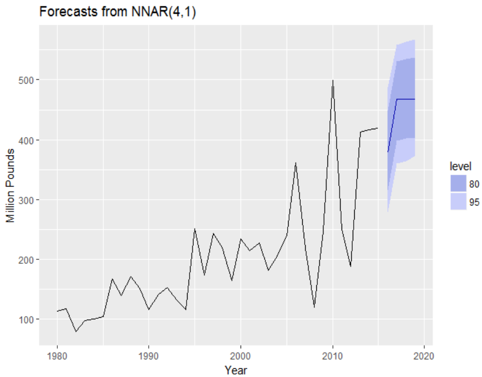
Figure 14. Arima, and NNAR Forecast results of domestic food utilization of both dry peas and lentils.
