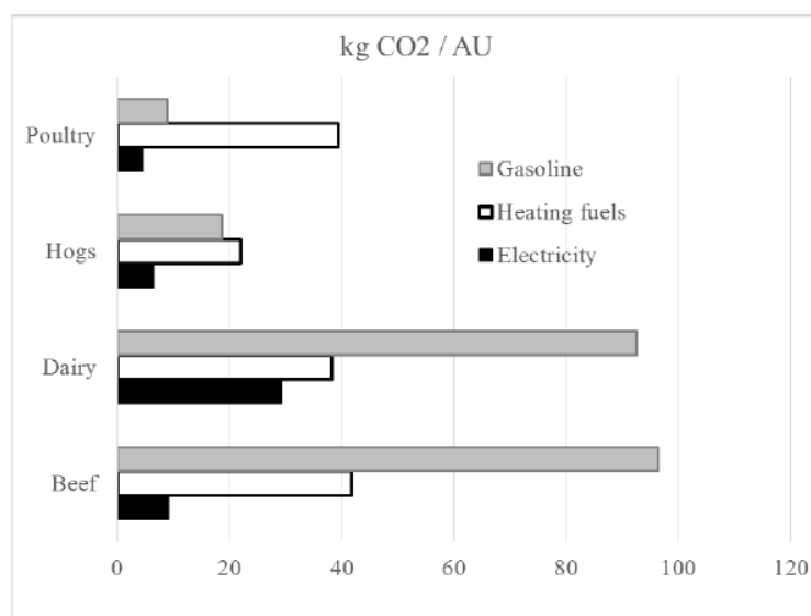
Figure 5. Distribution of fossil CO 2 emission rates over energy sources and livestock types expressed as CO 2 per Animal Unit (AU) for 2011
