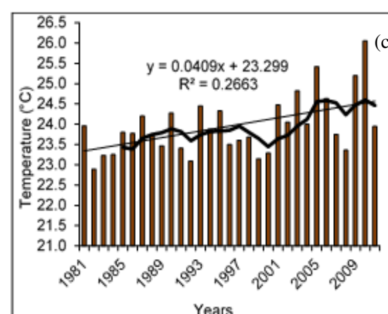
Figure 4: (a) Mean annual temperature trend, (b) mean season 1 (long rain) temperature trend, (c) mean season 2 (short rain) temperature trends, Luberizi catchment
