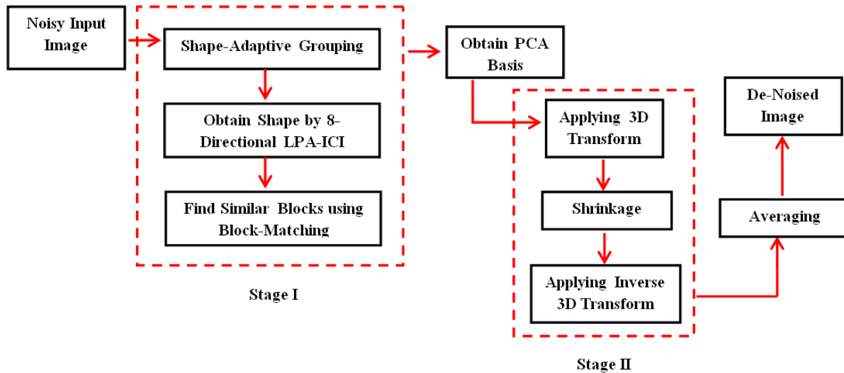
Figure 2: Block diagram of the proposed De-Noising algorithm
