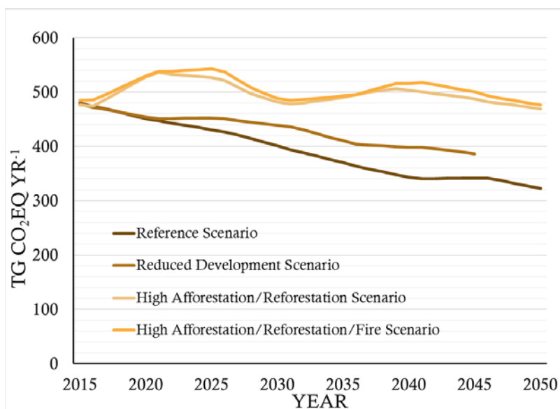
Figure 2. Projected annual carbon sequestration in forests of the coterminous U.S. under different policy scenarios (USDA 2016).
