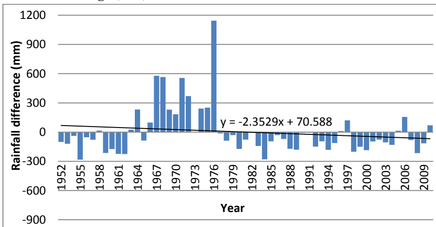
Figure 2: Year to year annual rainfall difference compared to 1952-2010 average (mm)
