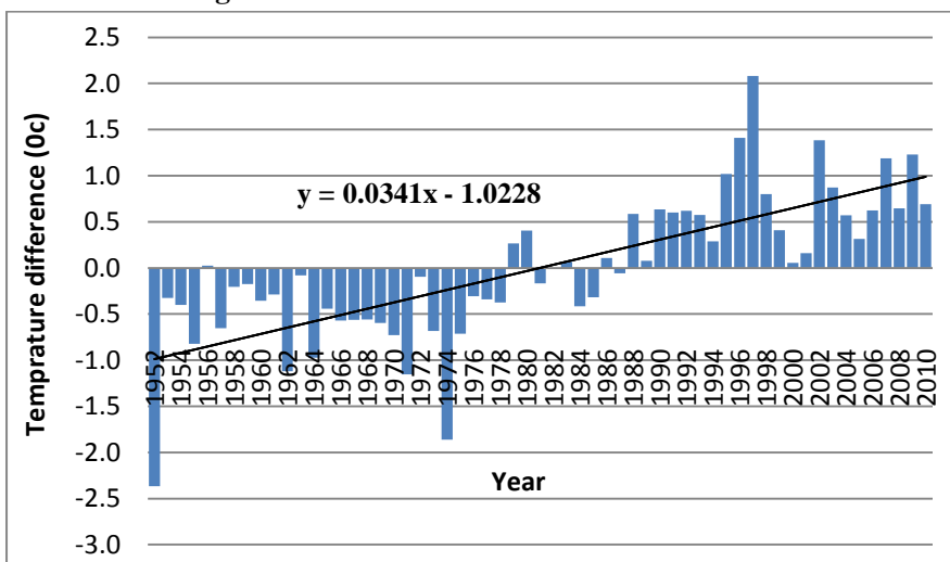
Figure 3: Year to year Temperature difference (°c) compared to 1952-2010 average
