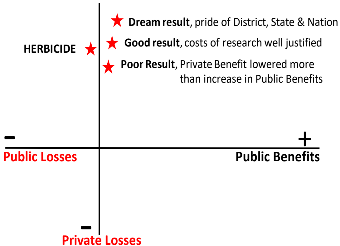
Figure 8. Research results in a public-private benefit framework (stylised). Presently, herbicides have important roles in vineyard weed management, being low-cost, easy to use and reliable. The rapid rise of herbicide resistance in weeds is a challenge to that reliability that will require integrating other means of weed management in vineyards as surely as it has in Australian broadacre agriculture. Source: authors
