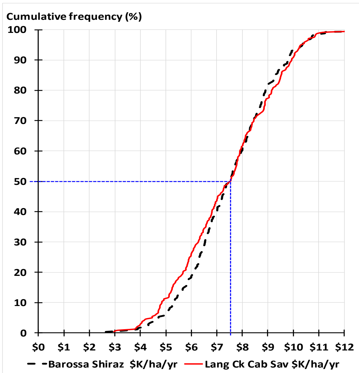
Figure 3. Annual gross revenues (price x yield) plotted as cumulative distribution functions based on simulated values as in Figure 2c.
