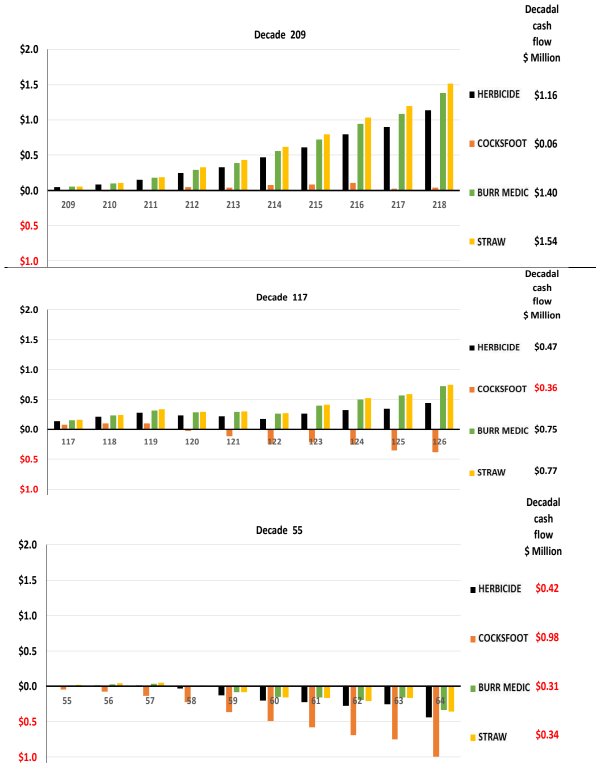
Figure 5. Examples of the annual and decadal cashflows (in $Millions) for a 50 ha Barossa vineyard with four under-vine treatments over three random decades (209, 117 and 55) among 231 stochastically simulated decades of varying fruit yields and prices, given $80K annual overhead costs. Source: compiled by authors
