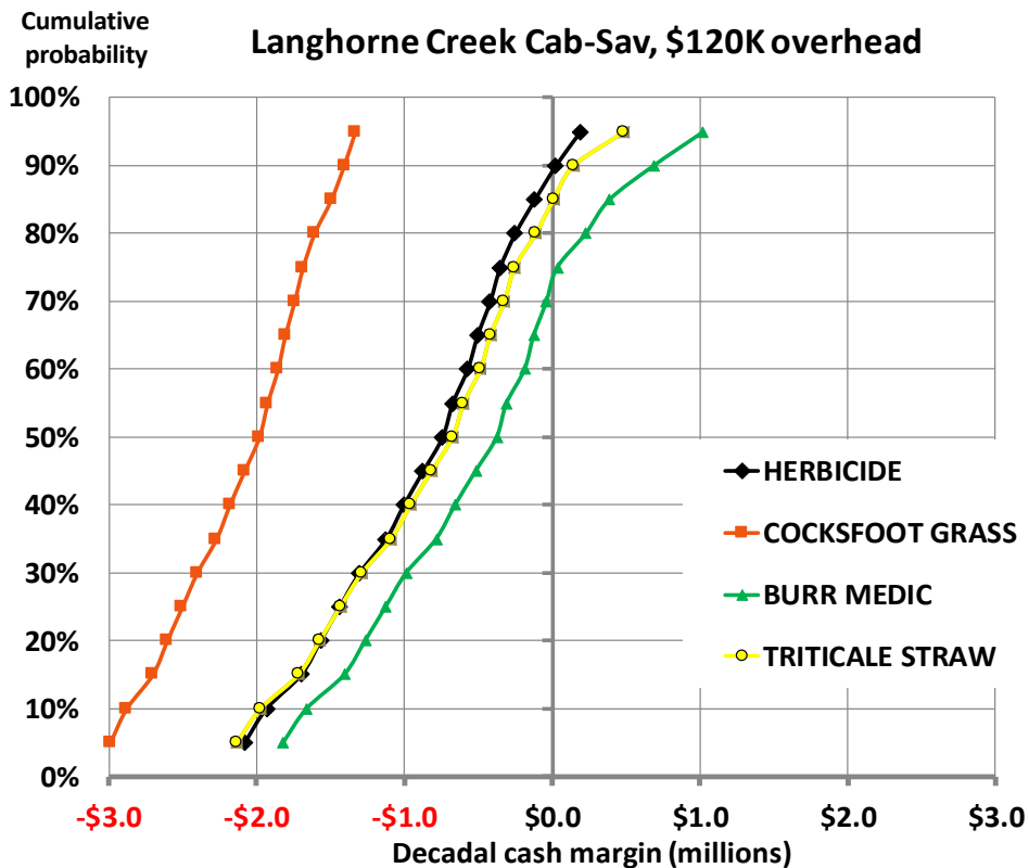
Figure 7. Cumulative distribution functions of decadal cash balance with four under-vine treatments in a 50 ha Langhorne Creek vineyard after interest, taxes, drawings and $80K and $120K annual overhead costs. Source: authors
