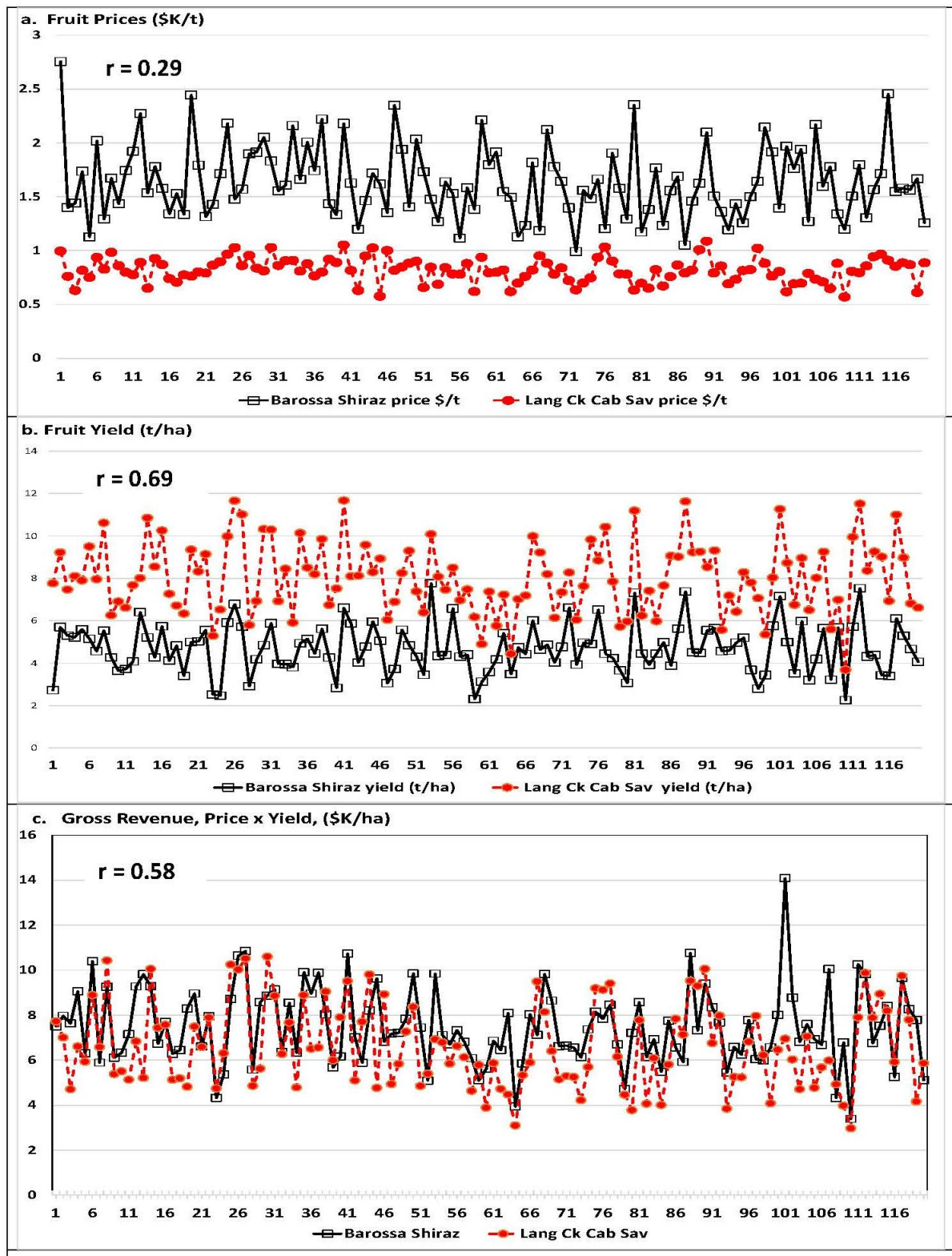
Figure 2. Simulated stochastic time series with correlated jointly-distributed random values for a) prices, b) yields and c) gross revenues of two variety / district combinations for 120 of 240 seasons with statistical properties modelled on 2006-2016. Source: derived from values in Table 1 by authors
