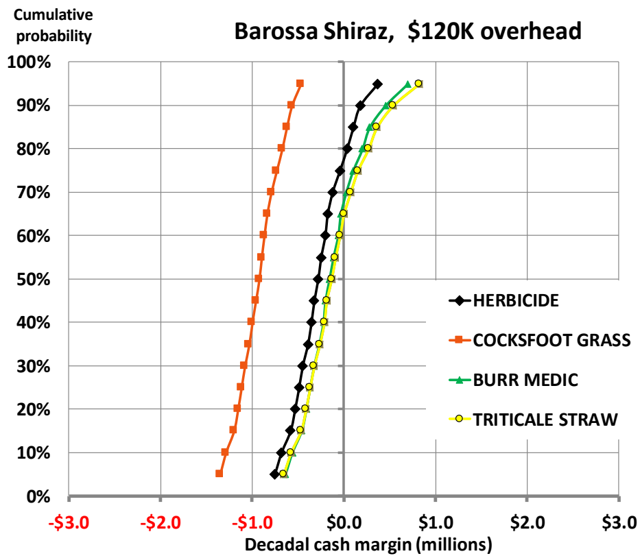
Figure 6. Cumulative distribution functions of decadal cash balance with four under-vine treatments on a 50 ha Barossa vineyard after interest, taxes, drawings and $80K and $120K annual overhead costs. Source: authors
