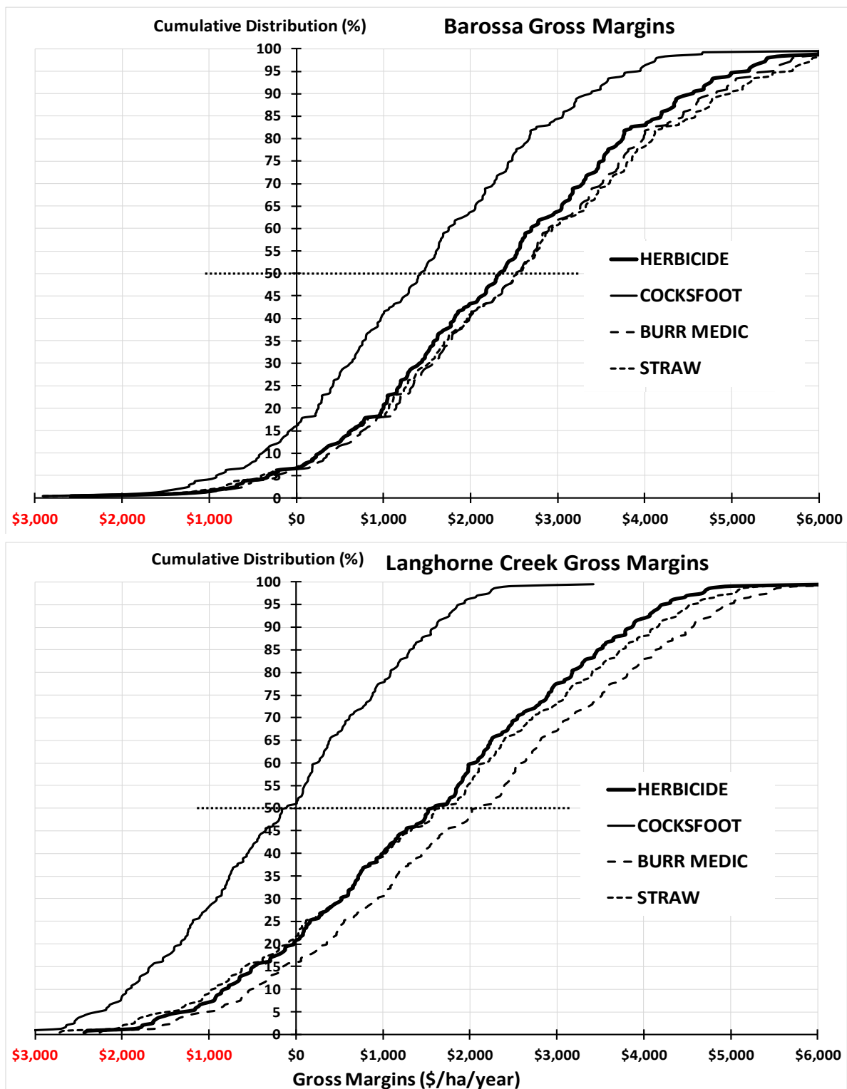
Figure 4. Cumulative distributions of Gross Margins: simulated as Gross Revenues minus Operational Costs ($/ha), before living costs, overheads, interest and taxes, of four under-vine treatments at experimental sites in two South Australian wine districts. Source: compiled by authors
