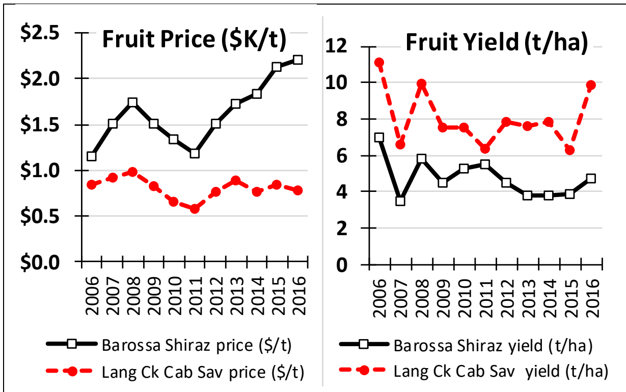
Figure 1. Reported fruit and price yields (2006-2016) for Shiraz grapes in the Barossa Valley and Cabernet Sauvignon grapes in the Langhorne Creek district. Source: Wine Australia (2016) South Australia Winegrape Crush Survey .
