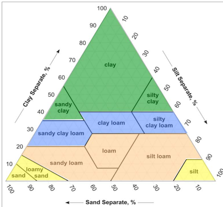
Figure 4. Soil Category Groups According to Clay Content
