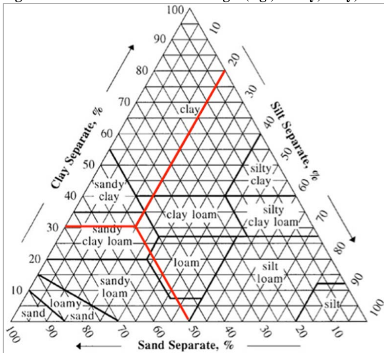
Figure 1. USDA Soil Texture Triangle (e.g., Sandy, Clay, Loam)
