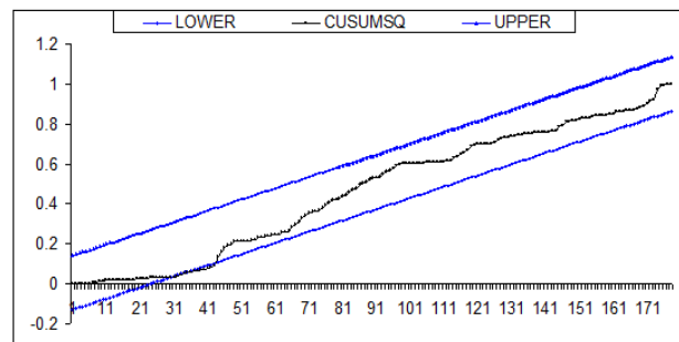
Figure 2: CUSUMQ test for farm and retail prices of chicken
