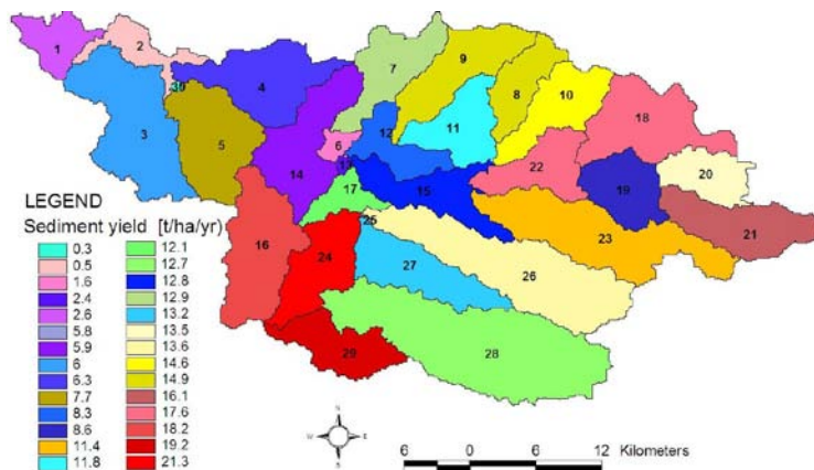
Figure 5 Spatial Distribution SWAT simulated average annual sediment yield by Micro Sub watershed(t/ha/yr). Number (1-30) are sub watershed numbers in Gumera watershed
