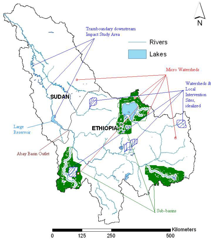
Fig. 1: Map showing the BNB and schematization of levels for erosion and sediment modeling
