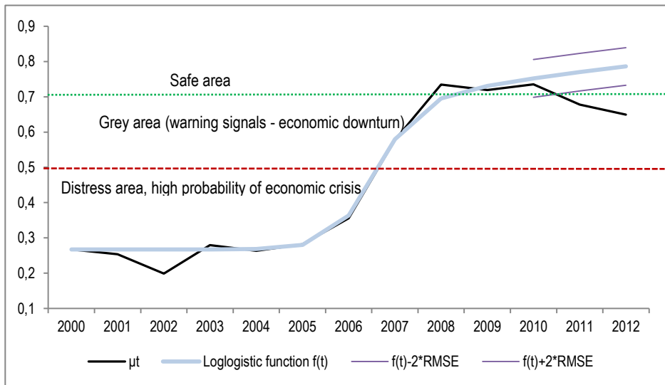
FIGURE 2. LOG-LOGISTIC FUNCTION ESTIMATION RESULTS
