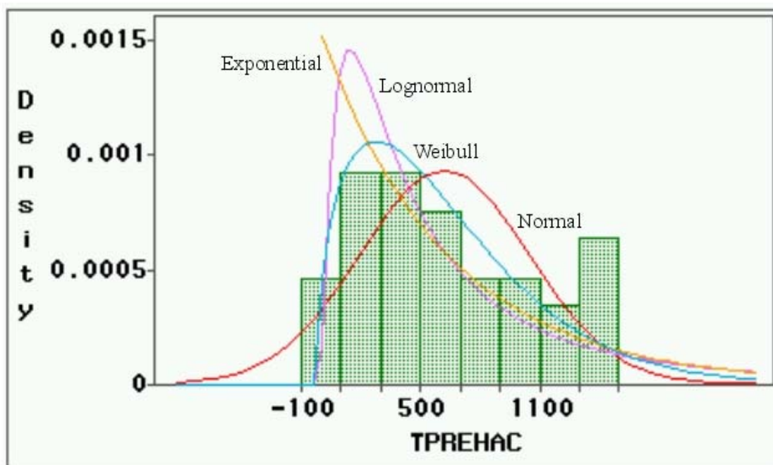
Figure 10. Parametric distributions fit to survival times for pre-HACCP period, all Class 1 recalls, 1994-Jan. 25, 1998.
