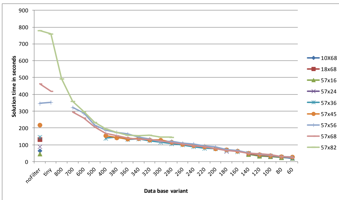
Graph 4: Solution time in seconds with differently detailed data bases and model configurations
