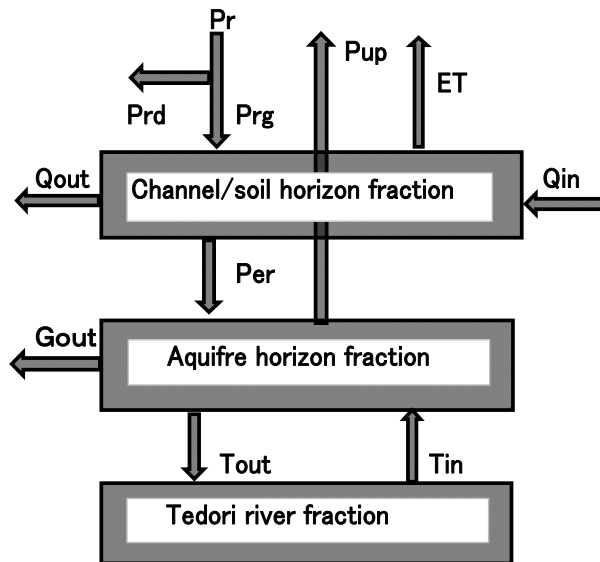
Figure 2. Water balance model and their symbols in the model
