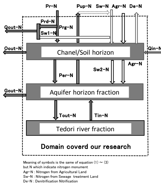
Figure 6. Nitrogen balance model and their symbols in the model
