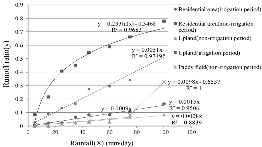
Figure 4. Relationship between precipitation and runoff ratio for different land use (Experimental equation for different land use determined by least square method)
