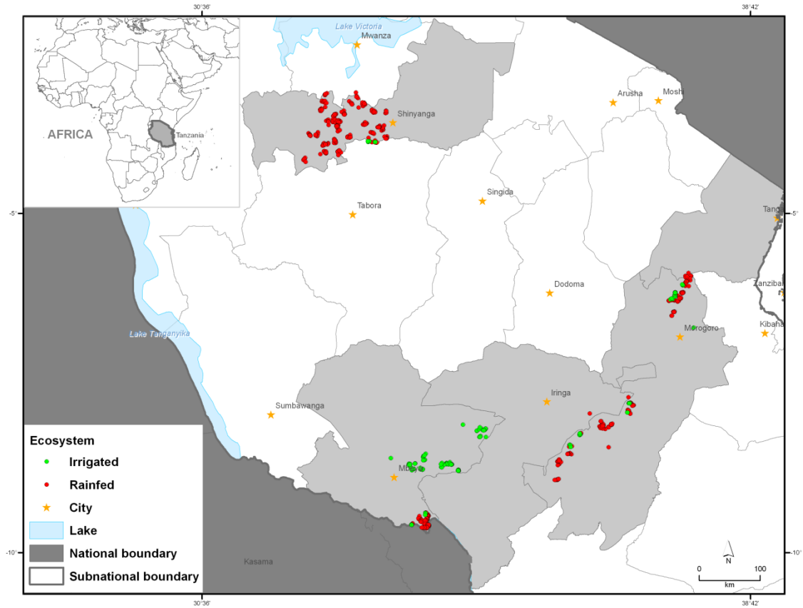
Fig. 3.1 Regions covered by extensive survey and location of the sample plots in Tanzania, by irrigation status
