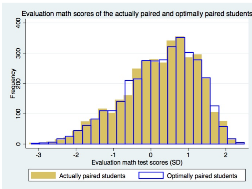
Figure 4. Comparison between the own standardized evaluation math score of the actually paired students in CAL treatment schools and the predicted own standardized evaluation math score of the optimally paired students
