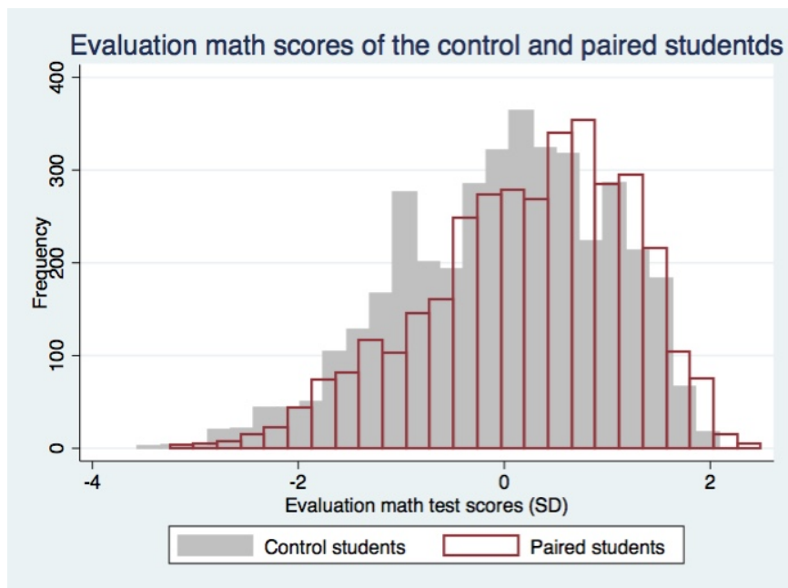
Figure 3. Comparison of own standardized evaluation math score between the control schools students and the paired students in CAL treatment schools
