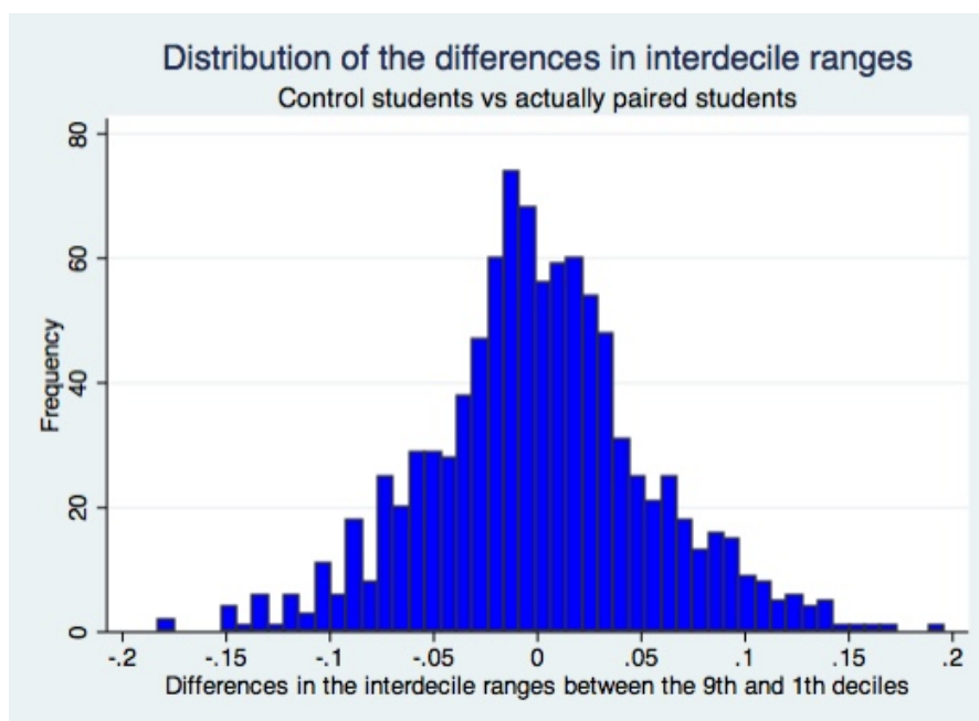
Figure 5. The simulated distribution of the difference in the interdecile ranges between the control school students and the paired students in the CAL treatment schools under the null that the score dispersion of the two groups is the same
