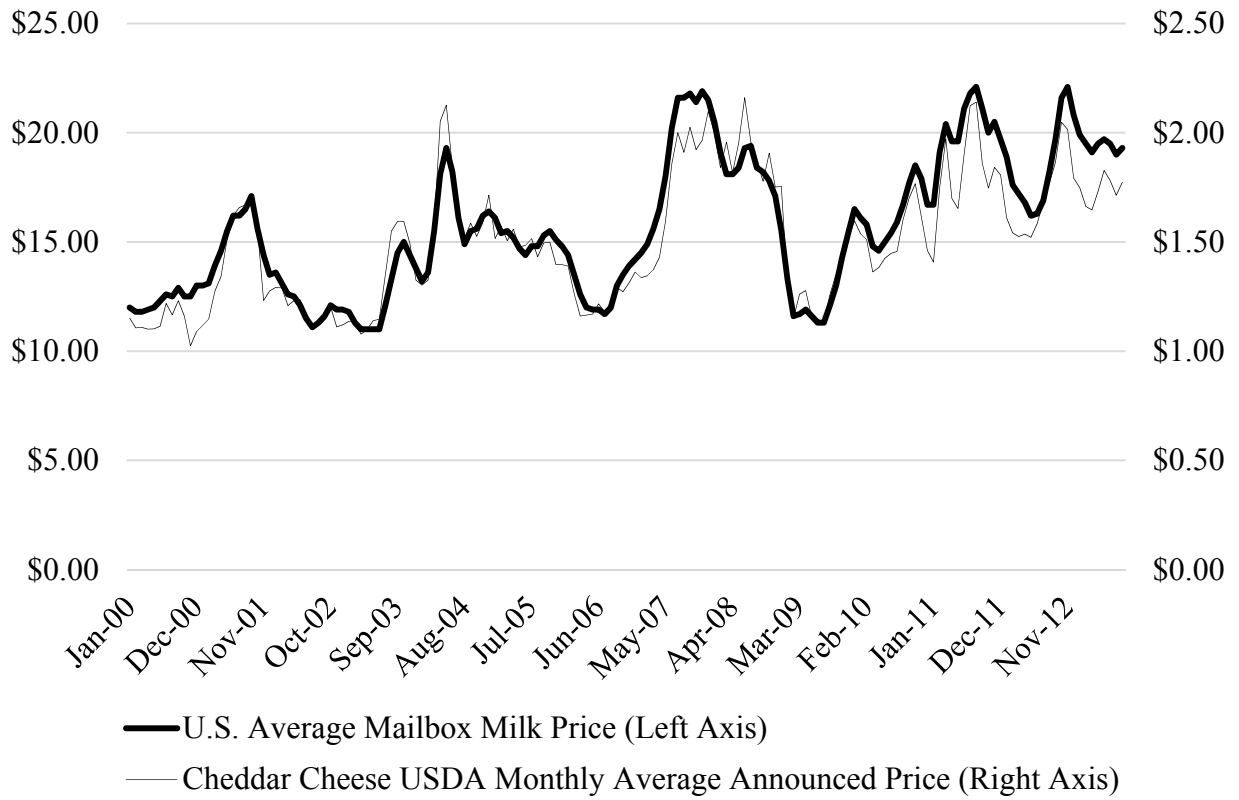
Figure 2. US. Mailbox Milk Price vs. Monthly Average Cheddar Cheese Price
