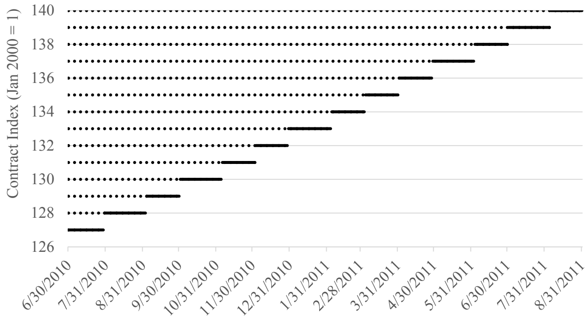
Figure 1. Constructing nearby futures price series
