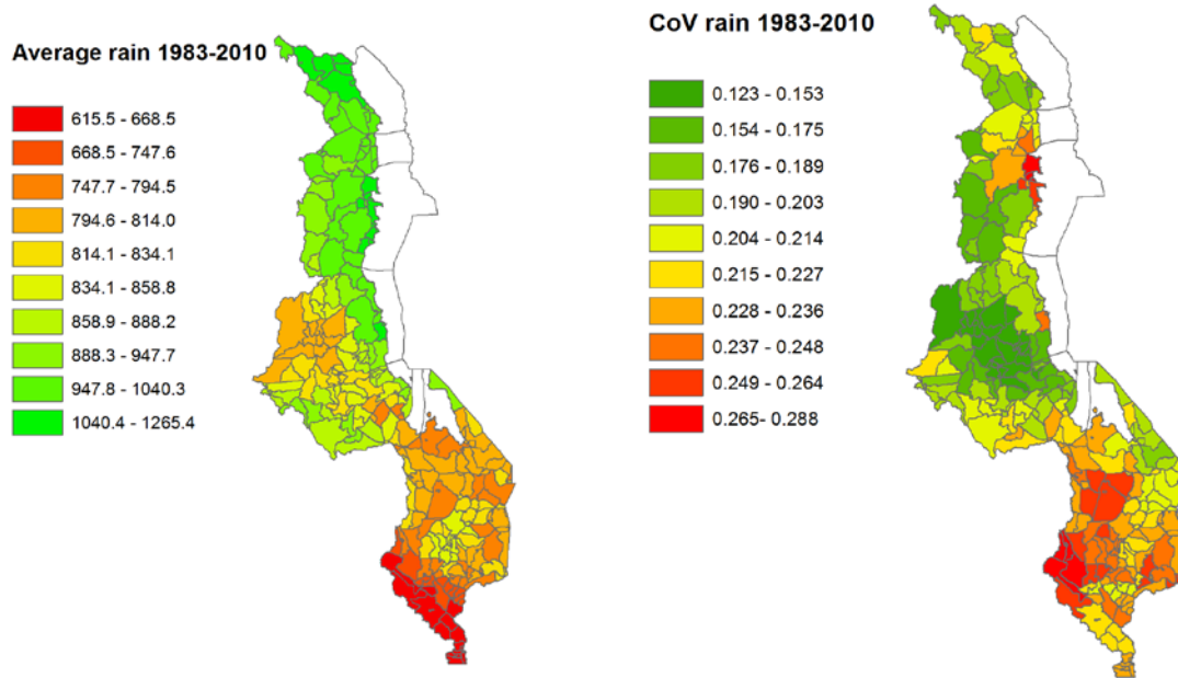
Figure 1. Total amount of rainfall and coefficient of variation (CoV) of rainfall (1983-2010)
