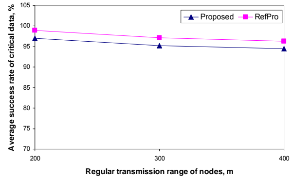
Fig. 7. Average success rate of critical data at different regular transmission ranges of nodes ( CH data rate = 10.0 pps, regular data rate = 1.0 pps).
