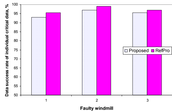
Fig. 9. Success rate of individual critical data ( CH data rate = 10.0 pps, regular data rate = 1.0 pps, regular transmission range = 300.0 m)
