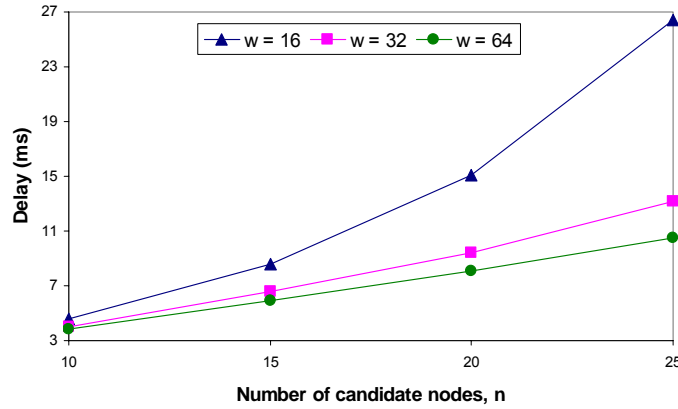
Fig. 3. CH selection delay at different number of candidate nodes
