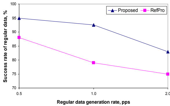
Fig. 6. Success rate of regular data at its different generation rates ( CH data rate = 10.0 pps, regular transmission range = 300.0 m).
