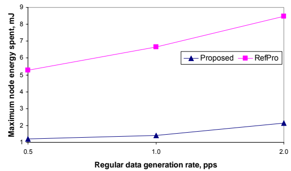
Fig. 11. Maximum node energy used at different generation rates of regular data ( CH data rate = 10.0 pps, regular transmission range = 300.0 m)
