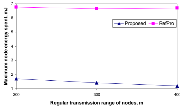
Fig. 10. Maximum node energy used at different regular transmission ranges of nodes ( CH data rate = 10.0 pps, regular data rate = 1.0 pps)
