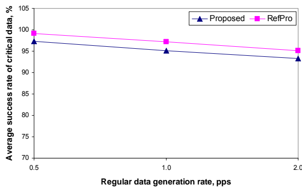
Fig. 8. Average success rate of critical data at different generation rates of regular data ( CH data rate = 10.0 pps, regular transmission range=300.0 m)
