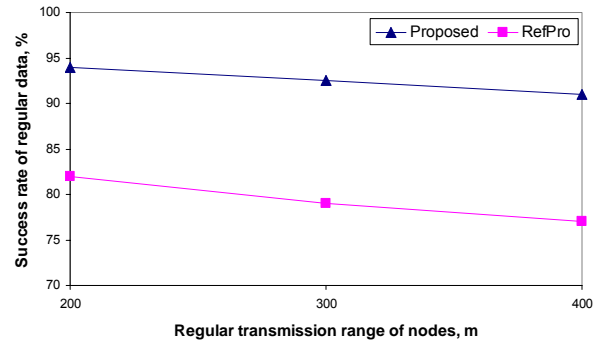
Fig. 5. Success rate of regular data at different regular transmission ranges of nodes ( CH data rate = 10.0\text{ pps} , regular data rate = 1.0\text{ pps} )
