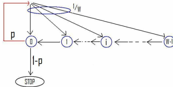
Fig. 2. Back-off process during CH selection
