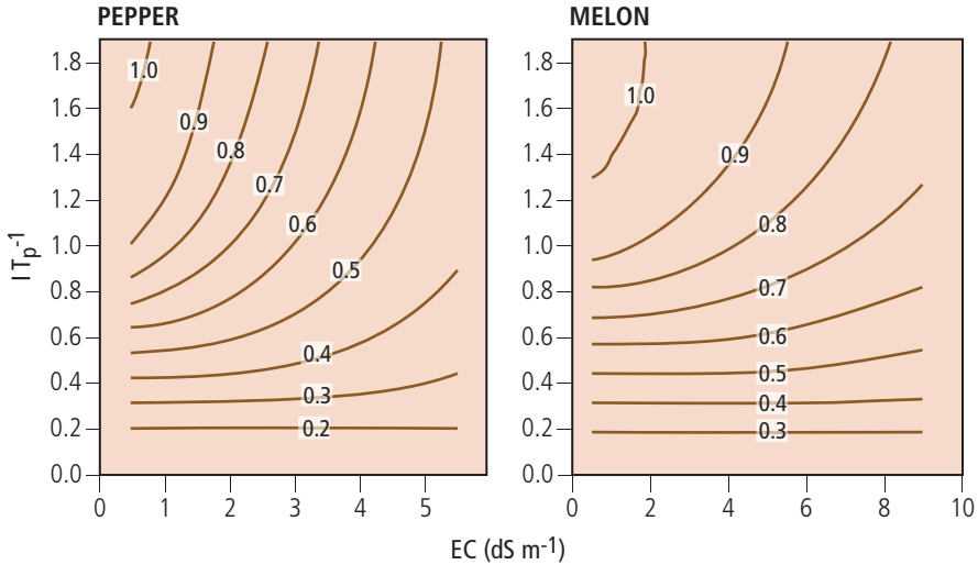
Figure 6. A compensation presentation of Iso-yield curves for irrigation water salinity (EC) and applied irrigation water quantity relative to climate demand ( I T_p^{-1} ) for pepper and melon crops. Curves were computed using the ANSWER model (Shani et al. , 2007). Isolines show 10% increases in relative yield.
