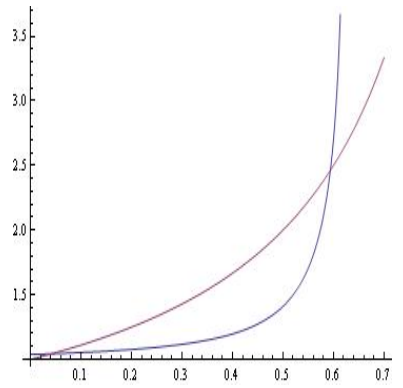
Figure 14: b = 50
