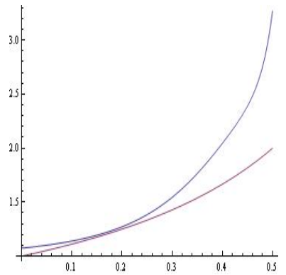
Figure 17: b = 50
