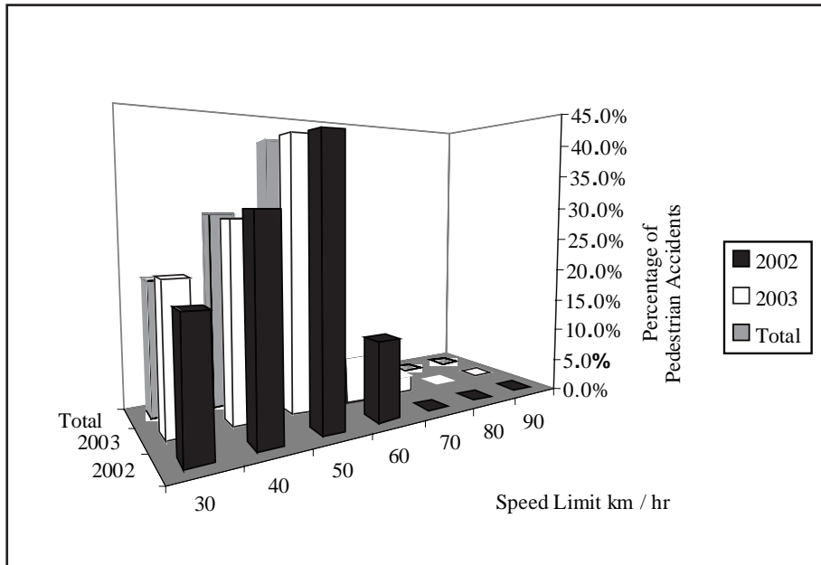
Figure 2: Pedestrian Accidents as Function of the Speed Limit
