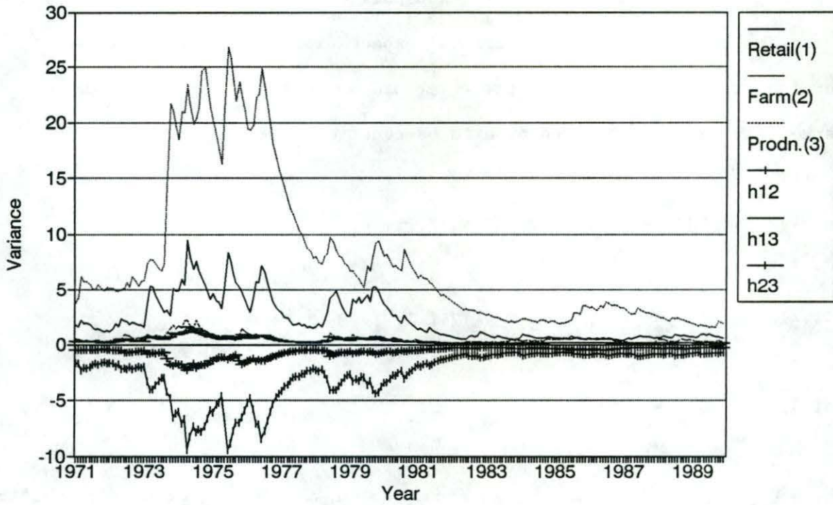
Figure 1. Time-Varying Conditional Variance Structure for the Estimated GARCH-M Model, 1971-89.
