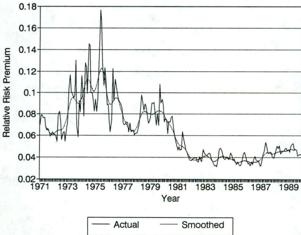
Figure 2. Time-Varying Relative Risk Premium in the Farm-Retail Margin.
