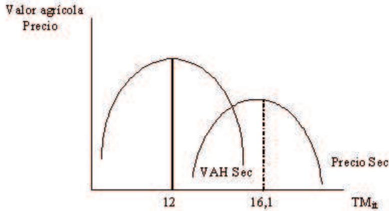
Figure 1: Effect of variation in the annual temperature regime
